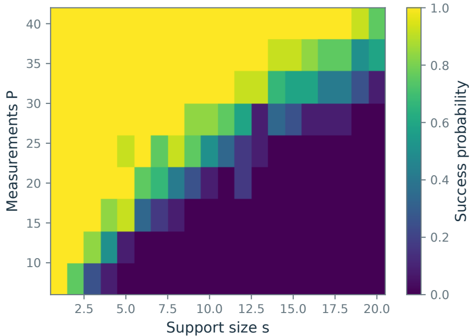
Empirical exact recovery (N=48)
