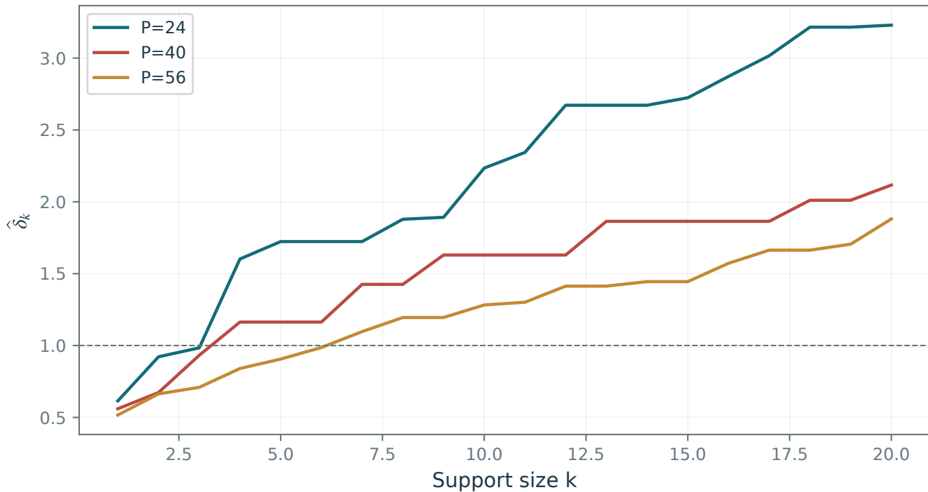
Sampled lower bounds on restricted isometry
