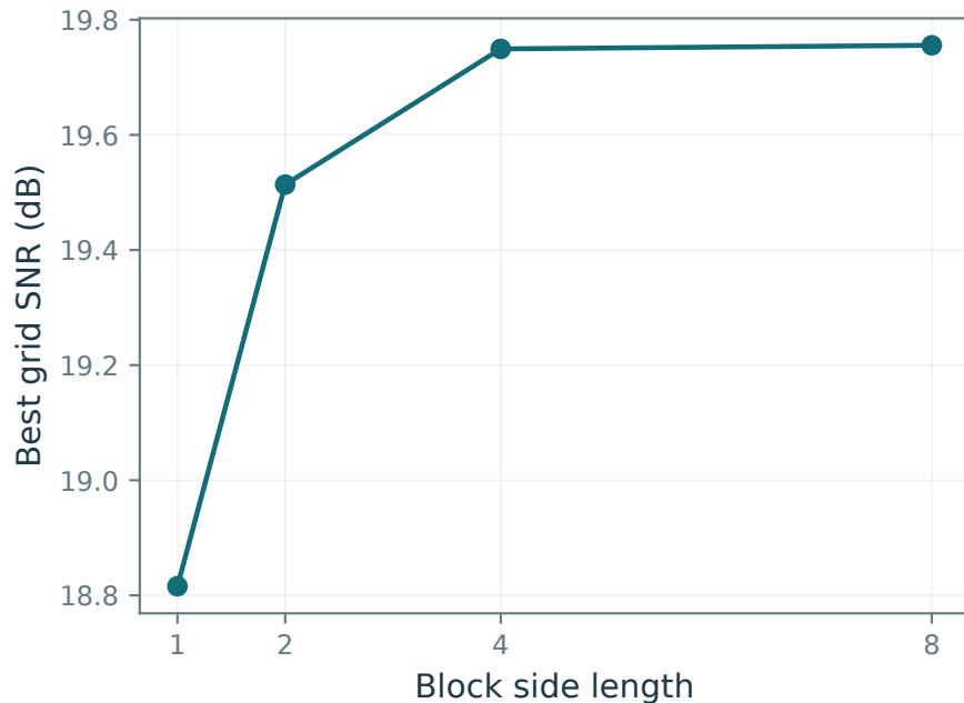
Stein rule: block-size comparison
