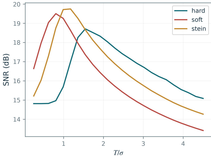
Rules on 4 × 4 blocks
