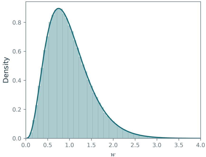
Mean-one multiplicative noise
