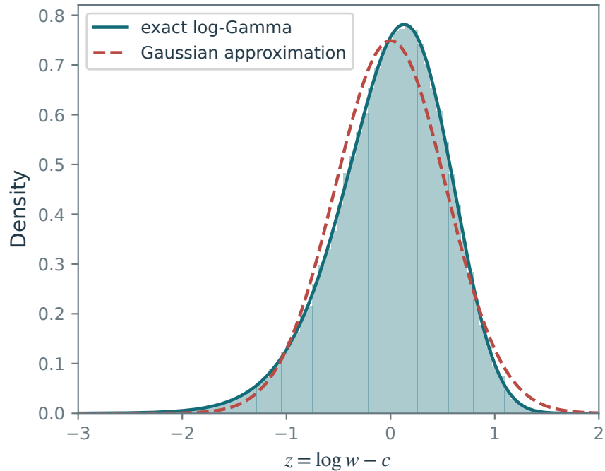
Centered additive log noise
