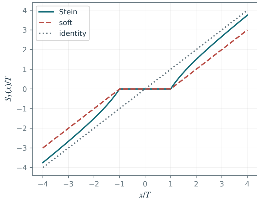
Stein thresholding
