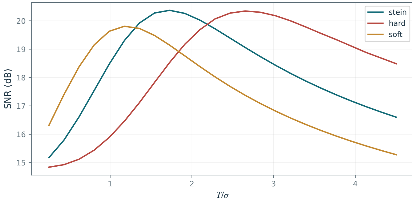
Stein and comparison shrinkage rules
