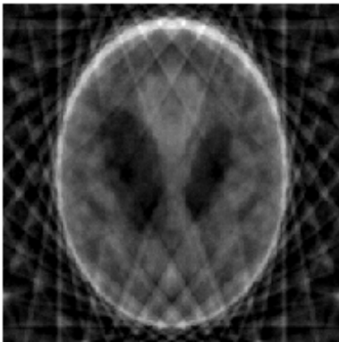
Pseudoinverse
