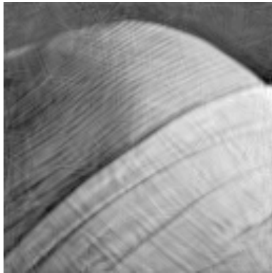
Curvelets \tilde{f}
