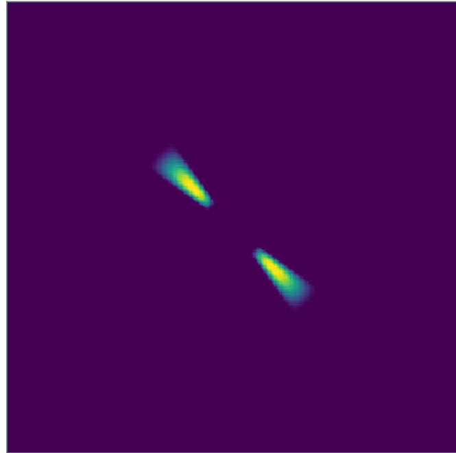
Two conjugate frequency wedges
