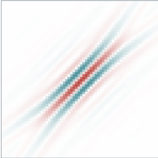
Real curvelet: spatial localization
