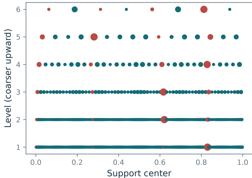
Haar supports meeting a jump (red)
