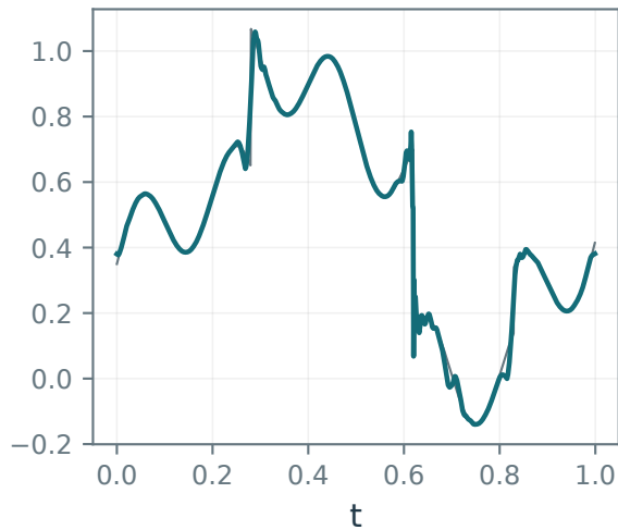
Largest db4 coefficients: M = 64
