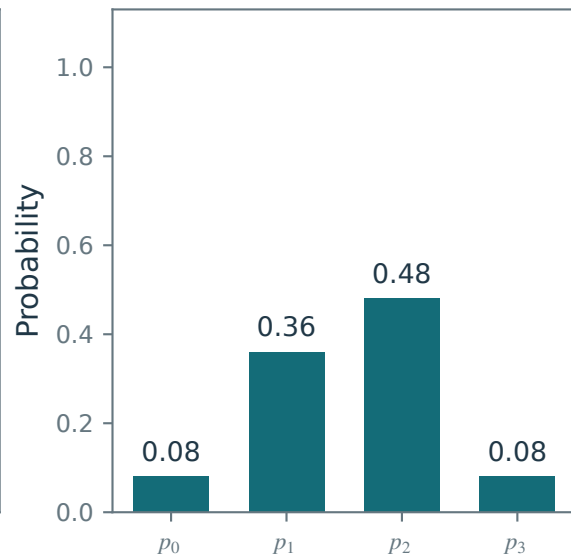
H(p) = 1.62 bits
