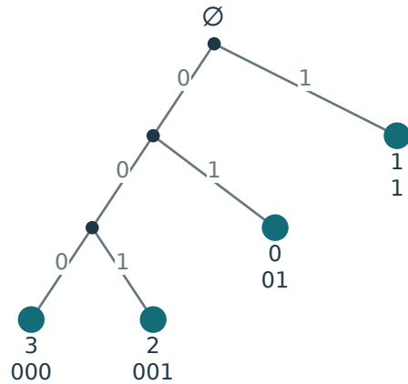
Resulting optimal prefix tree
