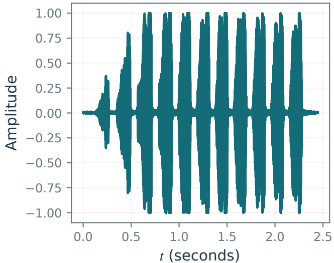
Sound: one time coordinate
