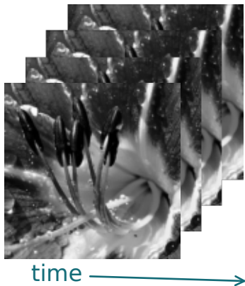
Video: space and time
