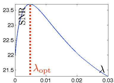
\ell^1 regularization
