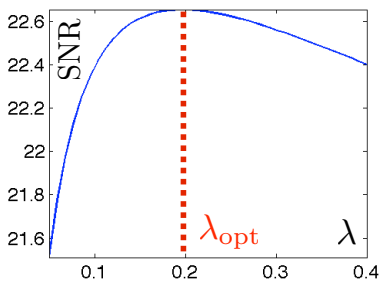
Sobolev regularization
