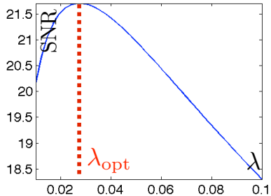
\ell^2 regularization
