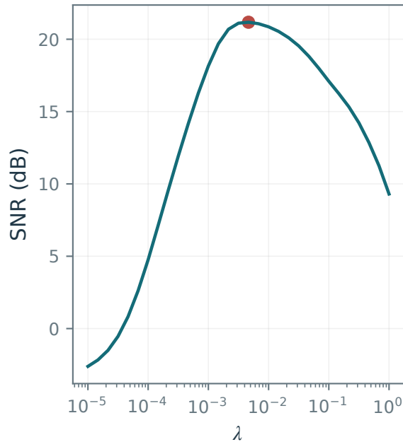
Orthogonal wavelets
