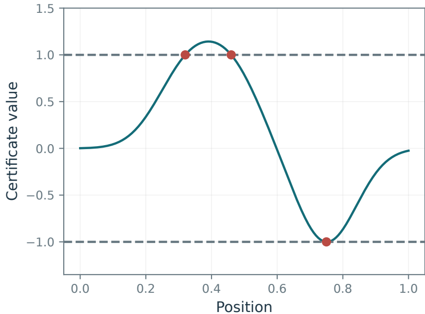
Fuchs \tilde{\eta}_F
