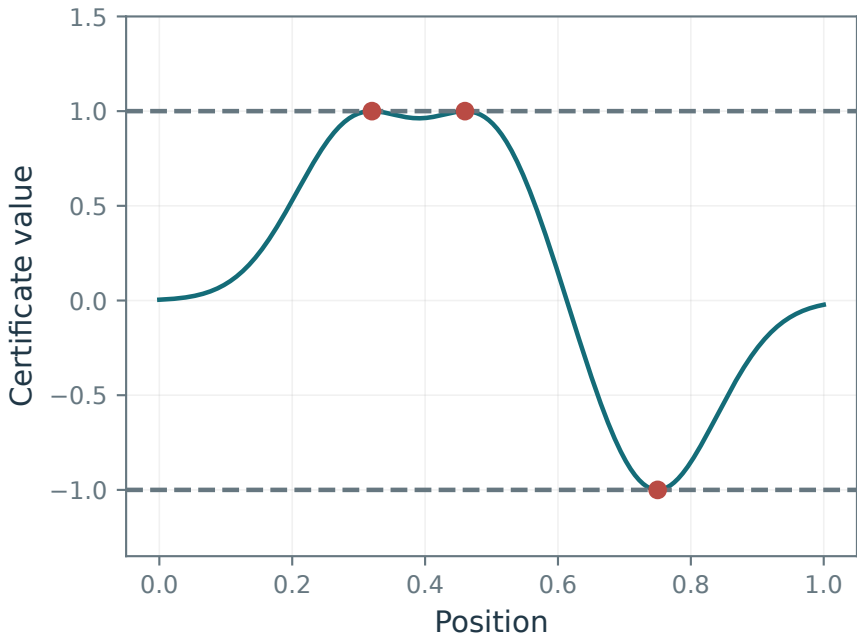
Vanishing derivative \tilde{\eta}_V
