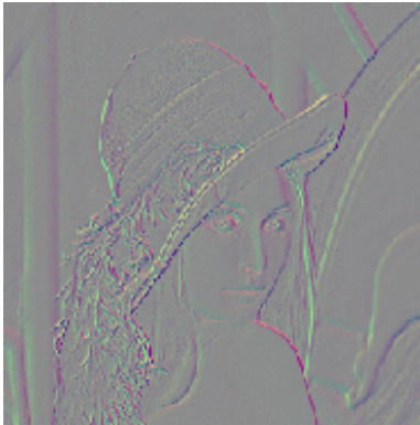
\nabla f
