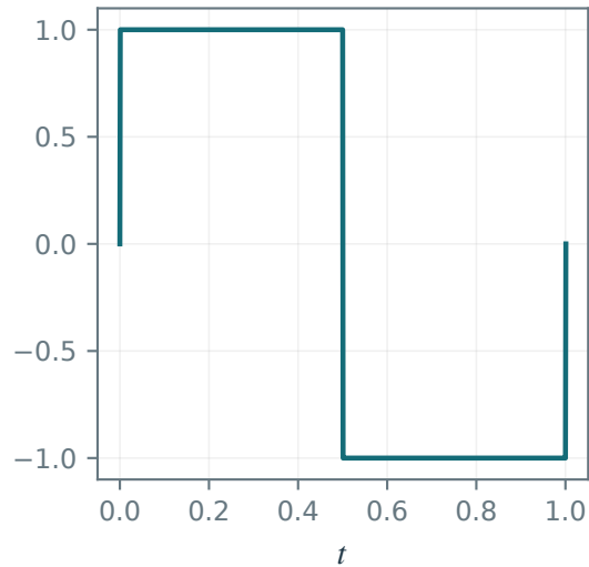
p = 1 vanishing moments
