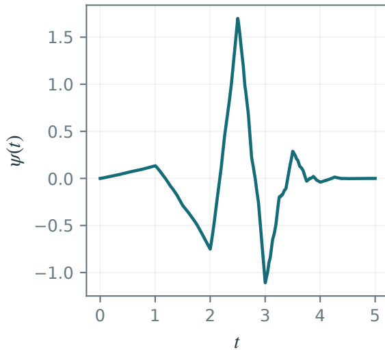
p = 3 vanishing moments
