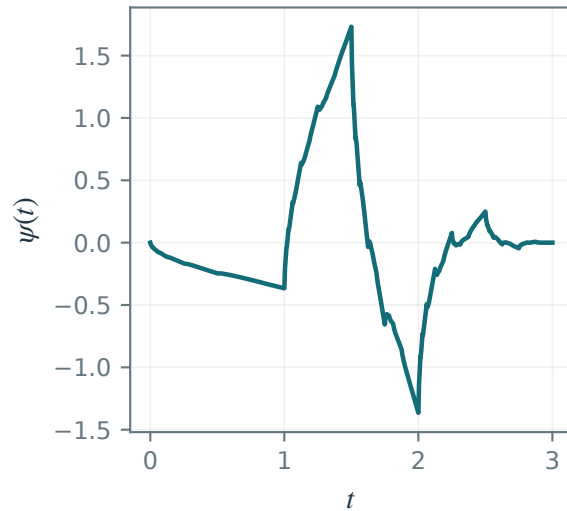
p = 2 vanishing moments
