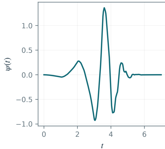
p = 4 vanishing moments
