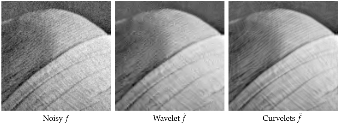
Figure 5.26. Comparison of translation-invariant wavelet denoising and curvelet denoising.
