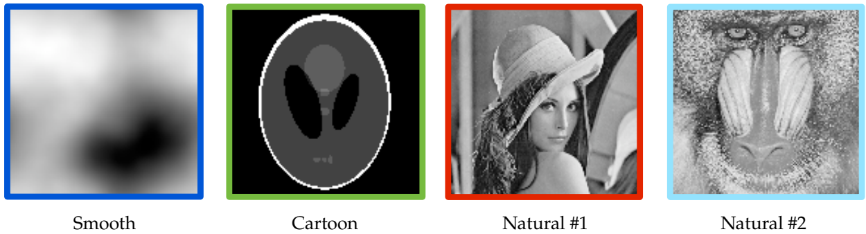
Figure 5.8. Test images with different types of structure.
