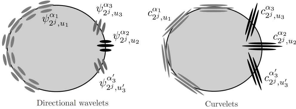
Figure 5.25. Wavelet (left) and curvelet (right) approximation of a cartoon image.
