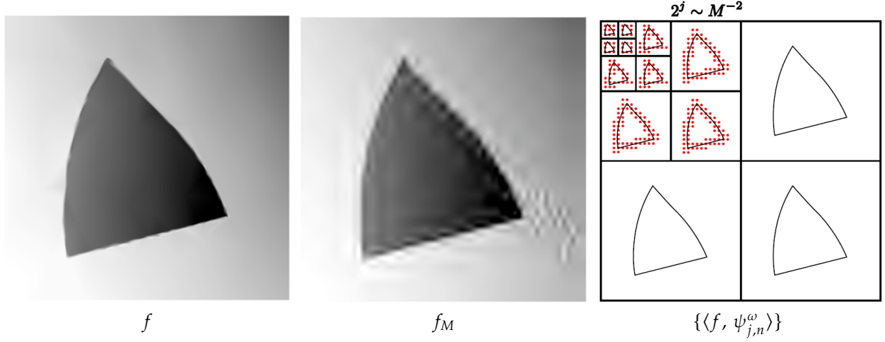
Figure 5.19. Wavelet approximation of a cartoon image.
