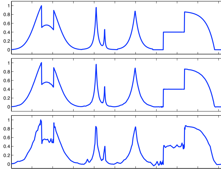
Figure 5.17. 1-D wavelet approximation.
