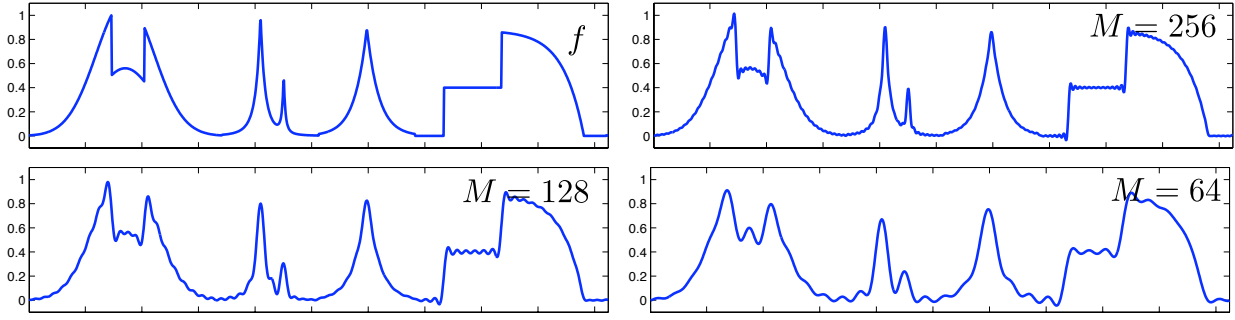
Figure 5.13. Fourier approximation of a signal.
