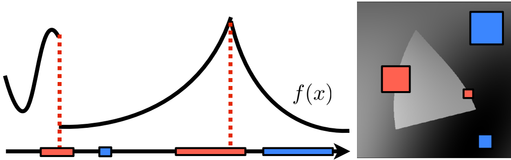
Figure 5.15. Singular and regular regions of a signal (left) and an image (right).
