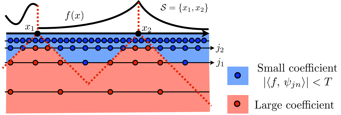
Figure 5.16. Segmentation of the wavelet coefficients into regular and singular parts.
