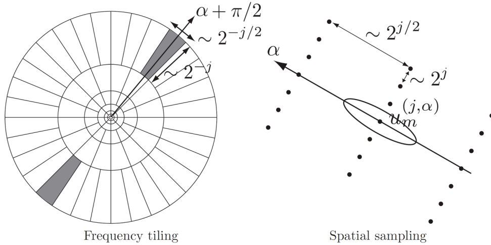
Figure 5.24. Sampling pattern for the curvelet positions.
