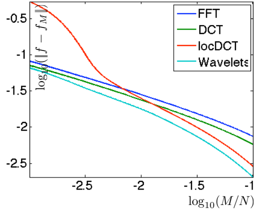
Figure 5.11. Comparison of approximation error decay for different bases.
