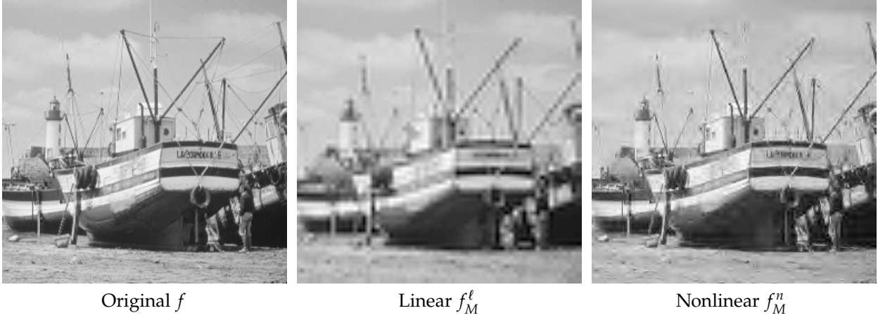
Figure 5.1. Linear versus nonlinear wavelet approximation.
