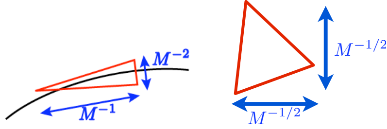
Figure 5.21. Anisotropic triangles near an edge (left) and approximately isotropic triangles away from edges (right).
