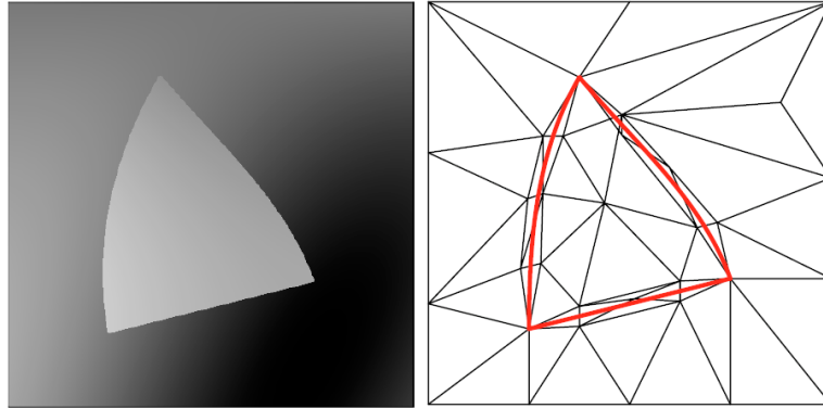
Figure 5.20. Left: cartoon image, right: adaptive triangulation.
