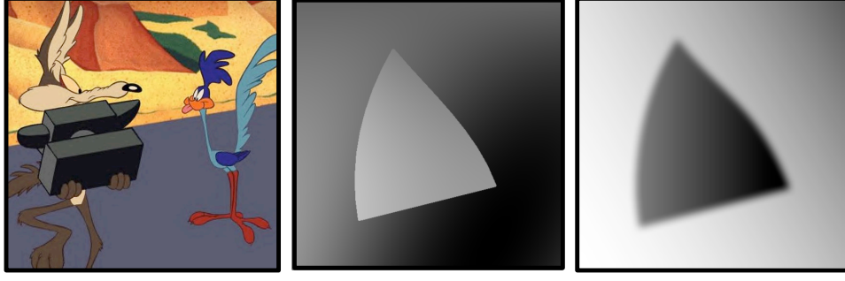
Figure 5.7. Examples of cartoon images: sharp discontinuities (left and center) and blurred edges (right).
