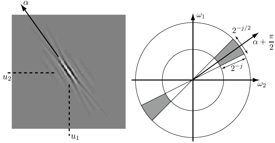
Figure 5.23. A curvelet c_m in space (left) and its localization in the Fourier domain (right).
