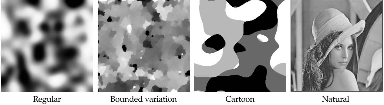
Figure 5.4. Examples of image models.
