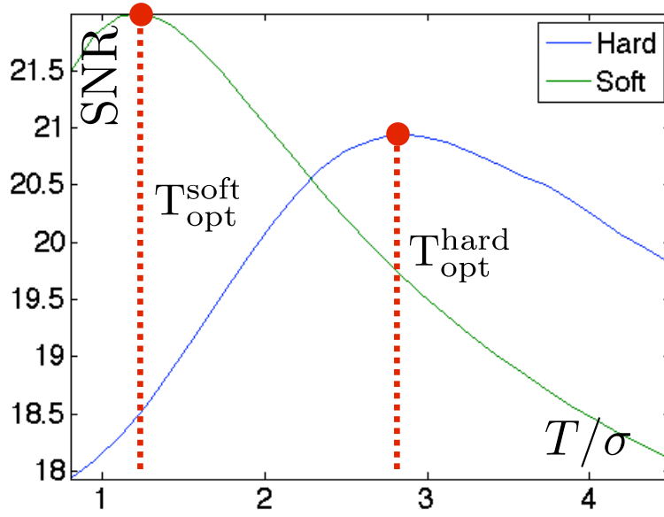
Figure 7.13. SNR as a function of T/\sigma for hard and soft thresholding.
