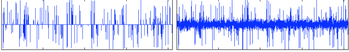
Figure 7.15. Left: clean sparse coefficients a_0 ; right: noisy coefficients a .
