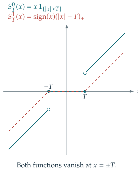
Figure 7.12. Hard and soft thresholding functions.
