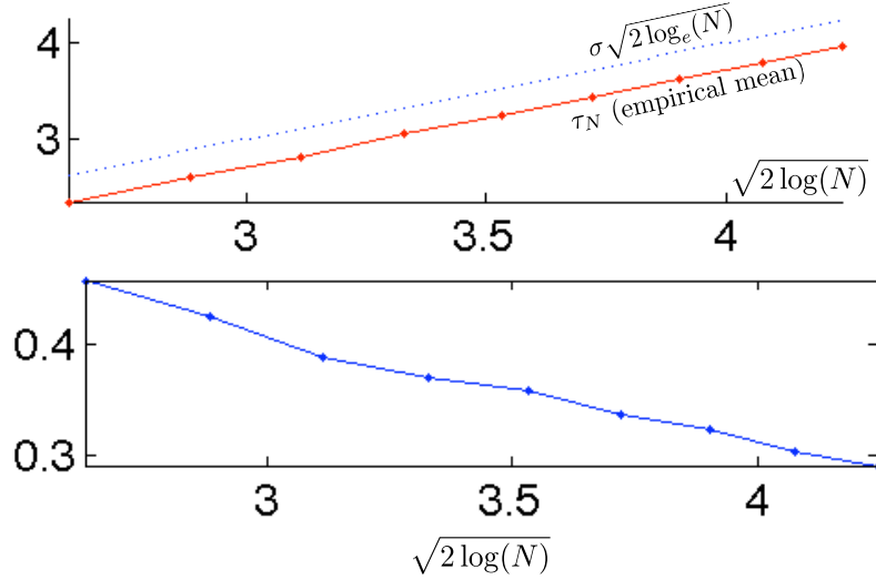
Figure 7.16. Empirical mean (top) and standard deviation (bottom) of the largest absolute Gaussian noise coefficient.
