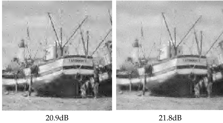
Figure 7.14. Comparison of hard (left) and soft (right) thresholding.
