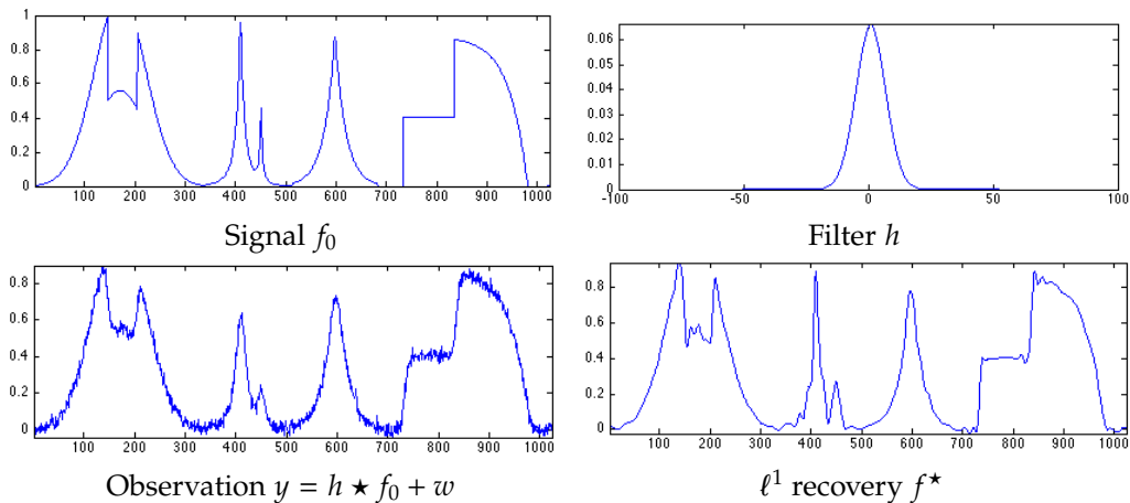
Figure 10.7. One-dimensional deconvolution with sparsity in an orthogonal wavelet basis.
