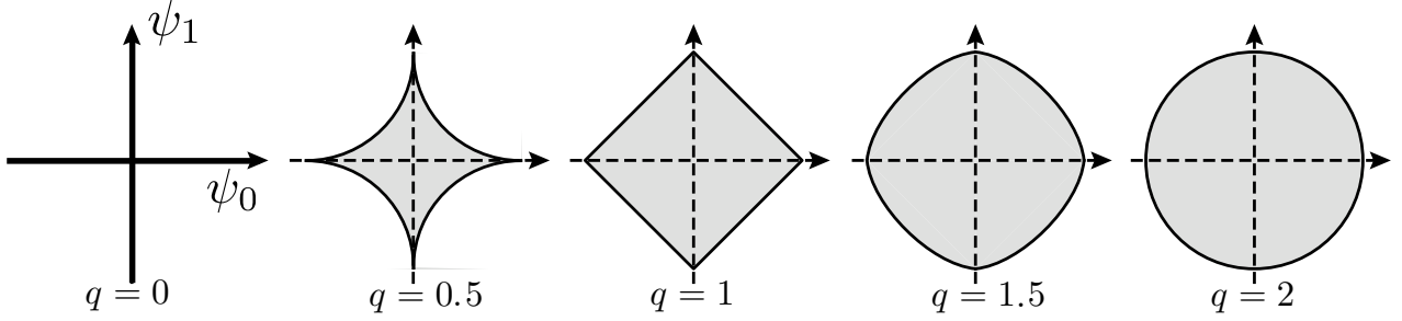
Figure 10.2. \ell^q balls \{x ; J_q(x) \leq 1\} for varying q .
