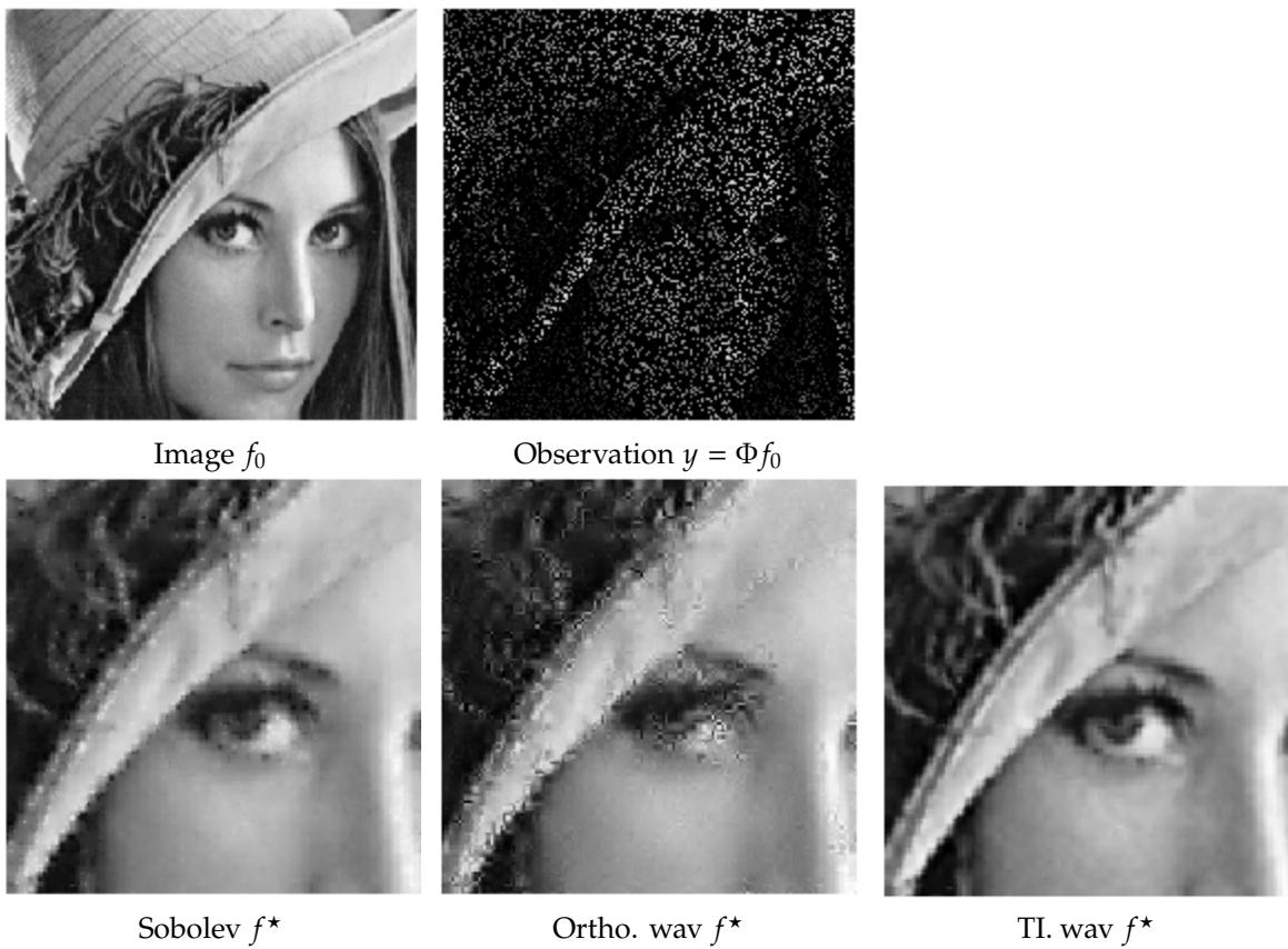
Figure 10.10. Inpainting with Sobolev and wavelet sparsity priors.
