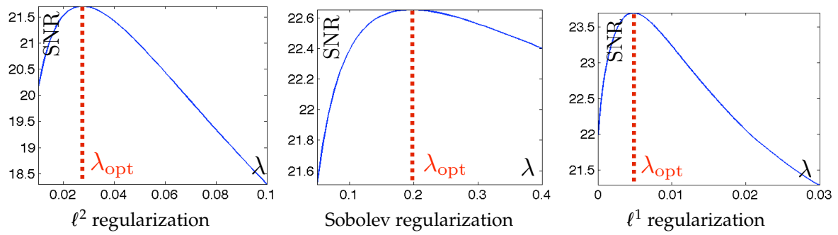
Figure 10.9. SNR as a function of \lambda .
