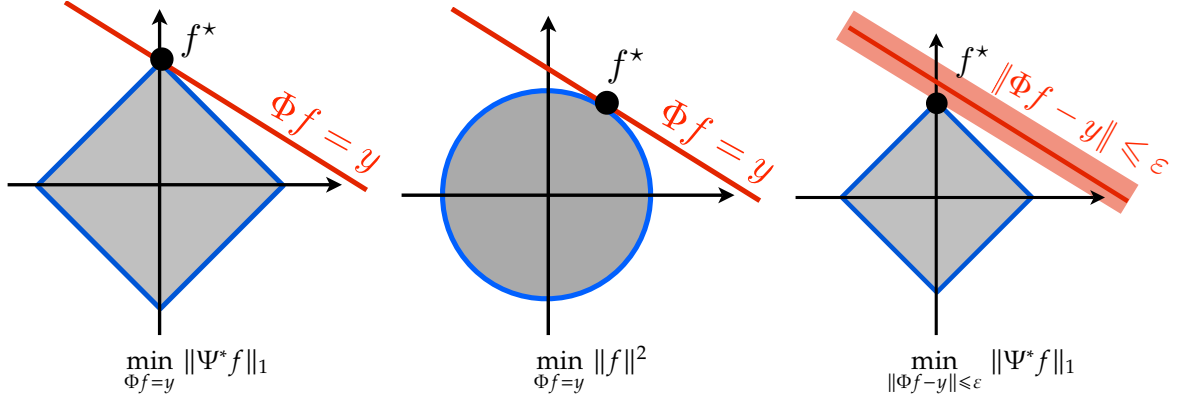
Figure 10.4. Geometry of convex optimization problems.
