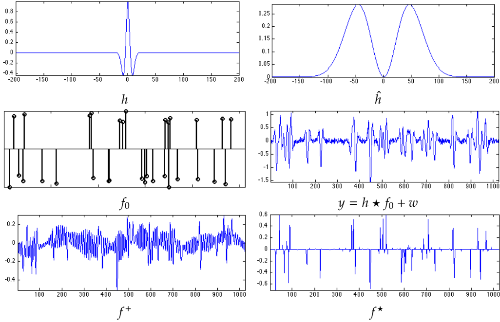
Figure 10.5. Sparse spike recovery by the pseudoinverse and by \ell^1 regularization.
