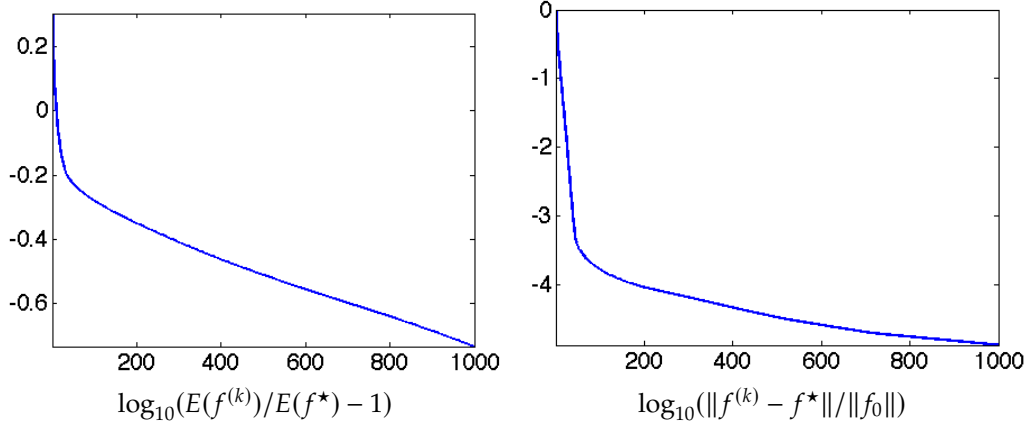
Figure 10.6. Convergence of the energy and iterates under iterative soft thresholding.
