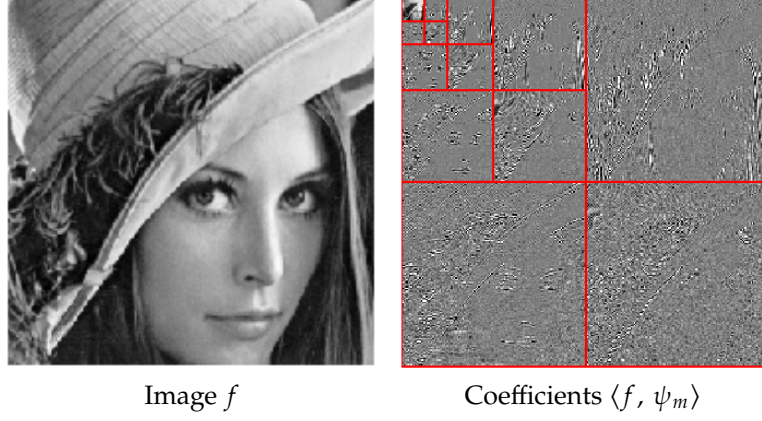
Figure 10.1. Most wavelet coefficients of a natural image have small magnitude.
