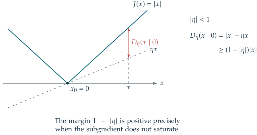
Figure 11.6. Bregman divergence controls the \ell^1 error on coordinates where \eta does not saturate.
