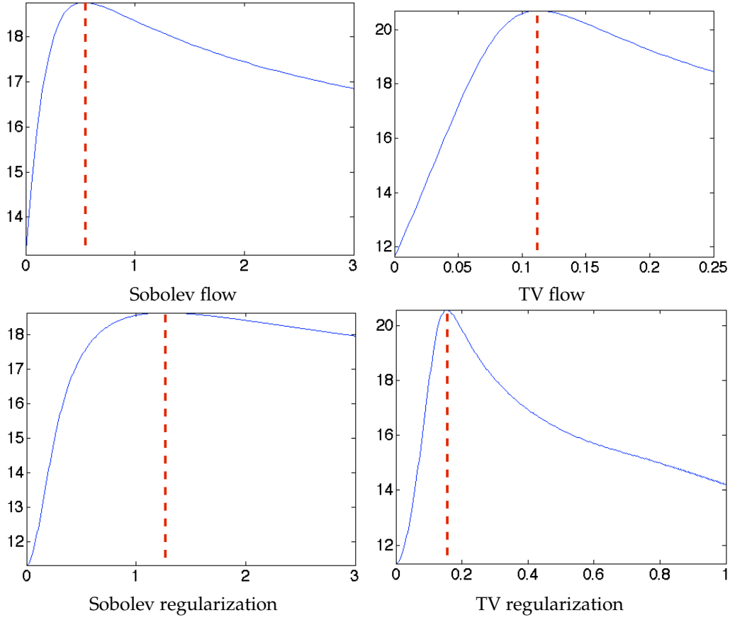
Figure 8.9. SNR as a function of time t for flows (top) and \lambda for regularization (bottom).
