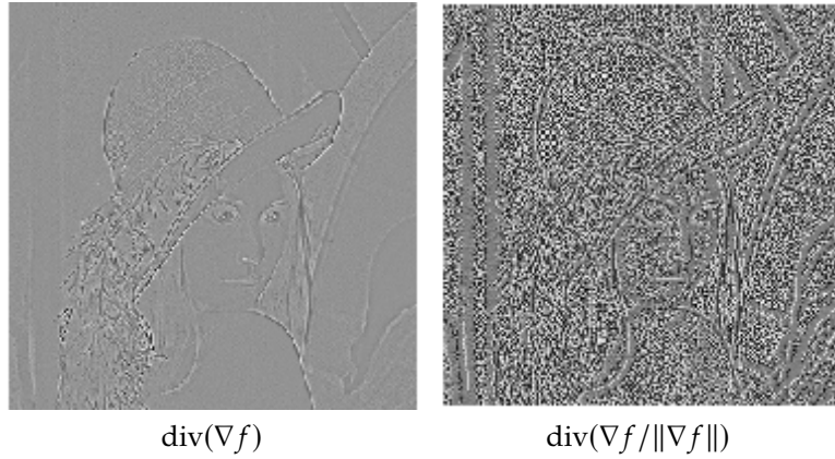
Figure 8.4. Discrete Laplacian (left) and negative discrete TV gradient (right).
