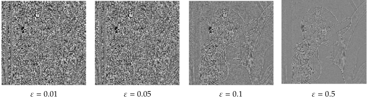
Figure 8.6. Regularized gradient norm \sqrt{\|\nabla f(x)\|^2 + \varepsilon^2} .
