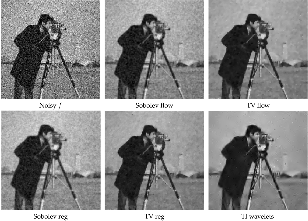
Figure 8.8. Denoising using PDE flows and regularization.
