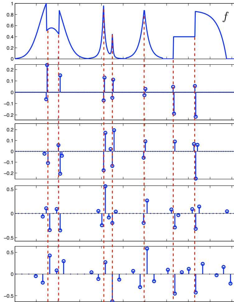
Figure 4.26. Location of large wavelet coefficients.
