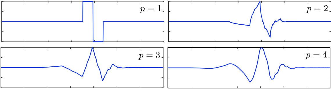
Figure 4.27. Daubechies mother wavelets \psi with increasing numbers p of vanishing moments.
