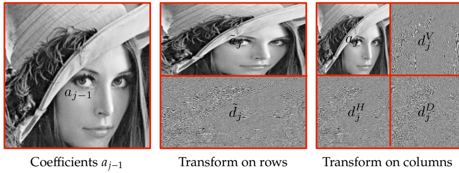
Figure 4.21. Forward 2-D filterbank step.
