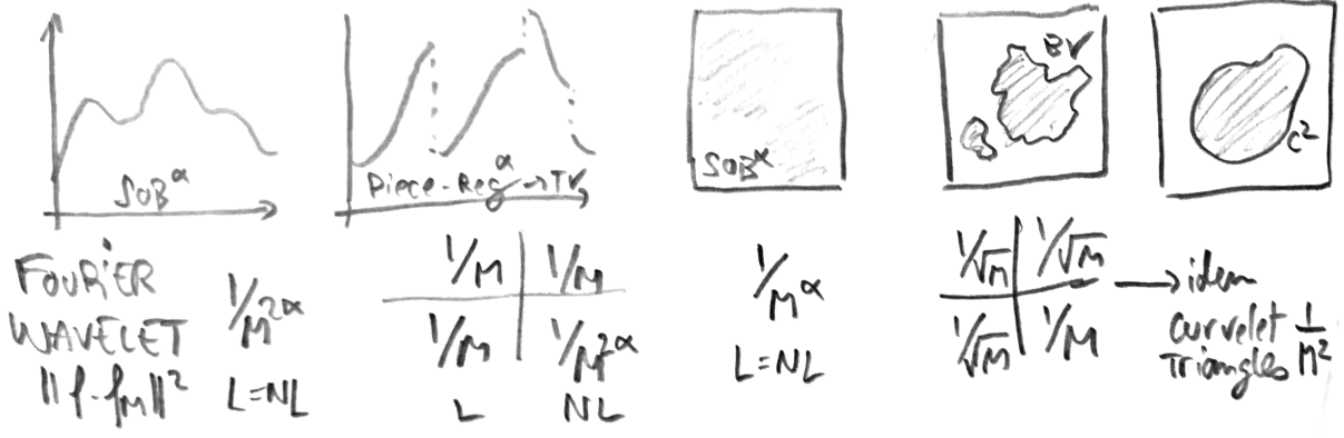
Figure 5.12. Summary of linear and nonlinear approximation rates \|f - f_M\|^2 for different classes of 1-D signals and images.
