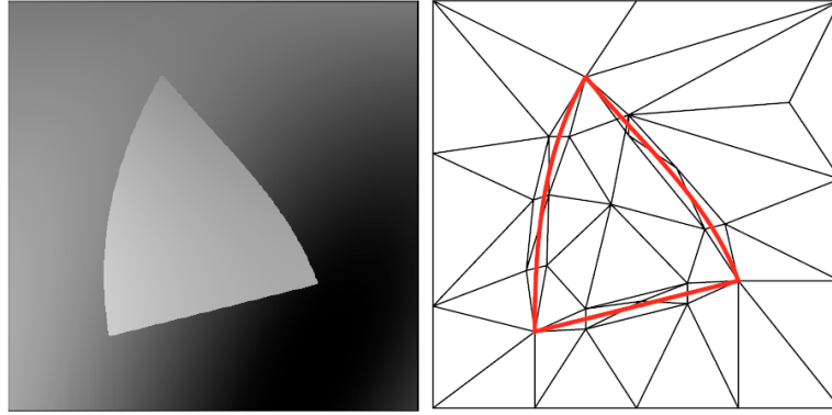
Figure 5.20. Left: cartoon image, right: adaptive triangulation.
