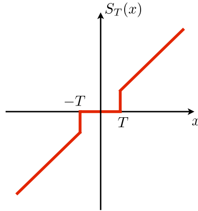
Figure 5.3. Hard thresholding.
