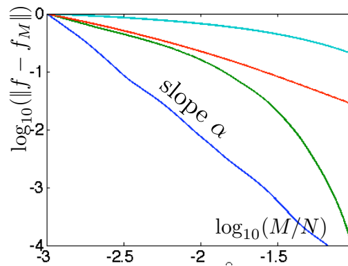
Figure 5.9. Wavelet approximation error for the images in Figure 5.8.
