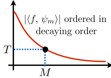
Figure 5.2. Ordered coefficient magnitudes and the threshold used for nonlinear approximation.
