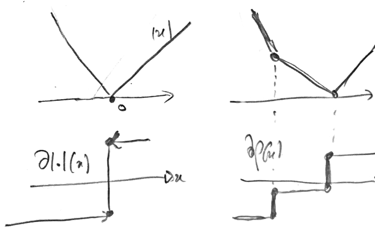
Figure 18.3. Subdifferential of the absolute value and a piecewise affine convex function.
