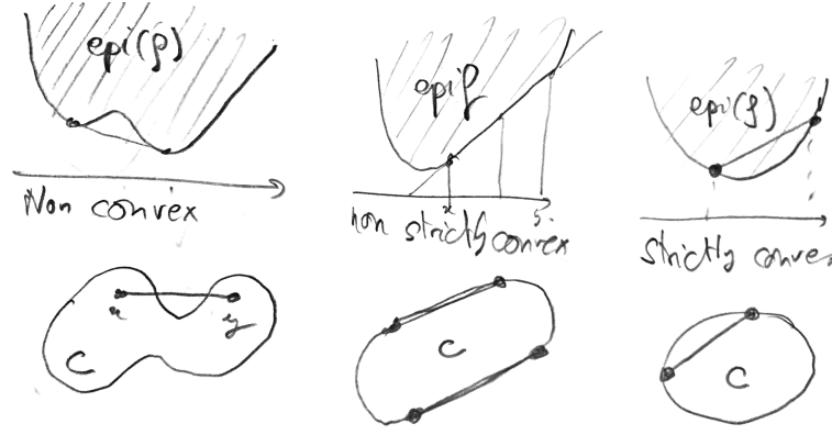
Figure 18.1. Convexity and strict convexity for functions and sets.
