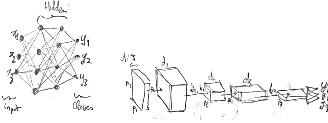
Figure 17.1. Left: fully connected network. Right: convolutional neural network.
