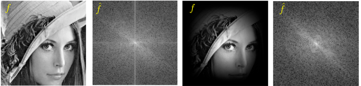
Figure 2.17. 2-D Fourier analysis of an image (left), and attenuation of the periodicity artifact using masking (right).
