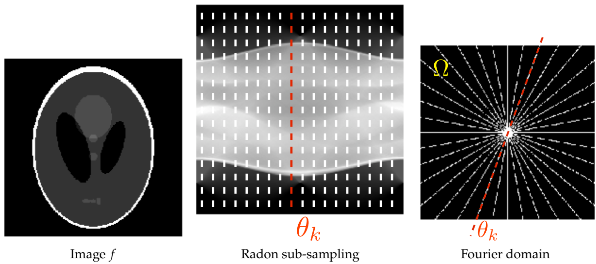
Figure 9.8. Partial Fourier measurements.
