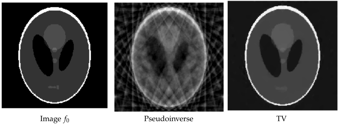
Figure 9.10. Tomographic reconstruction with total variation regularization.
