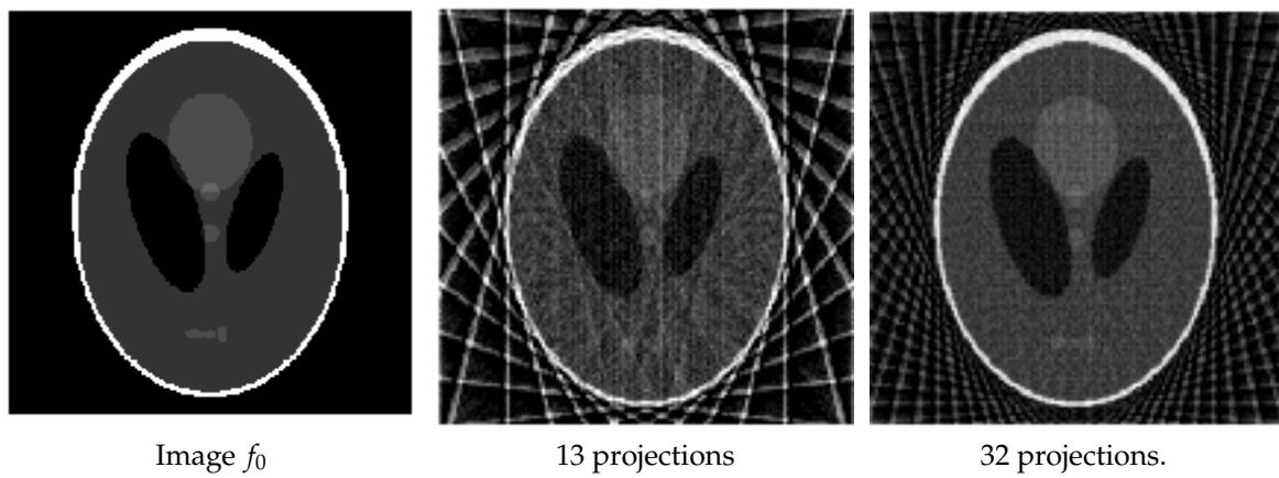
Figure 9.9. Pseudoinverse reconstruction from partial Radon projections.
