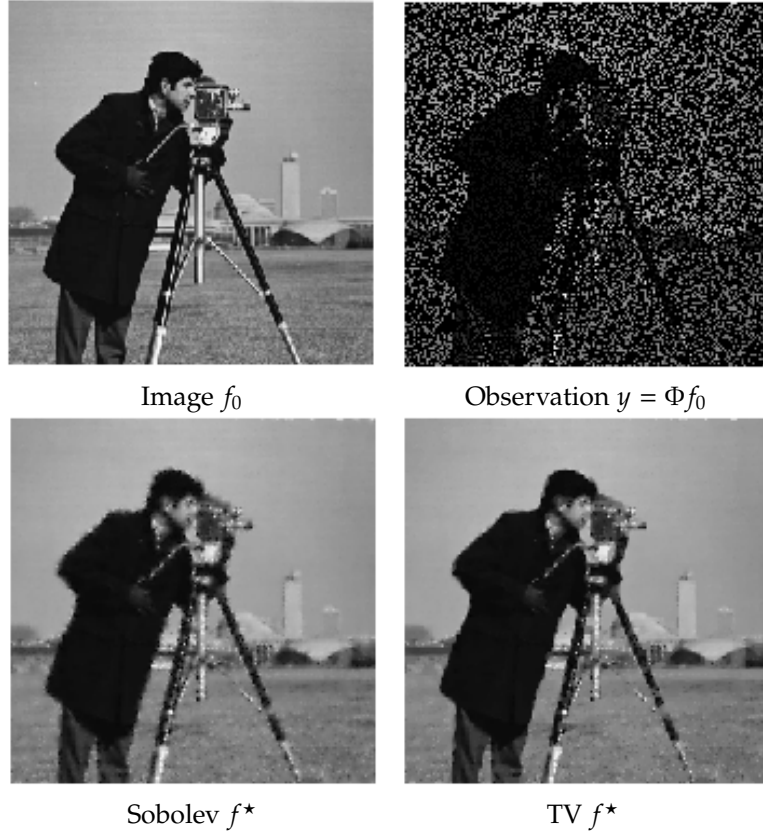
Figure 9.6. Inpainting with Sobolev and TV regularization.
