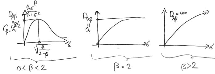
Figure 9.3. Bounding \lambda \frac{\sigma^\beta}{\lambda + \sigma^2} \leq D_{\lambda, \beta} .
