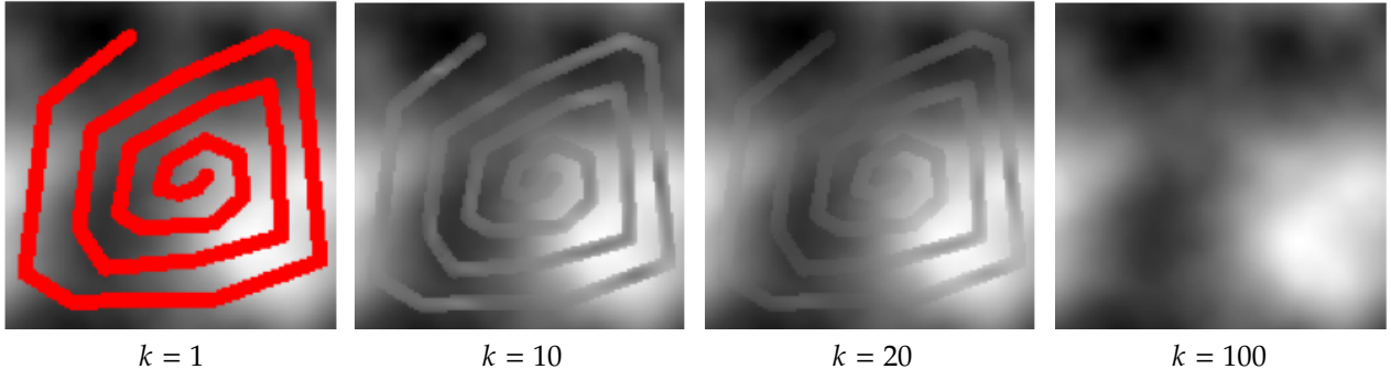
Figure 9.4. Sobolev projected gradient descent algorithm.
