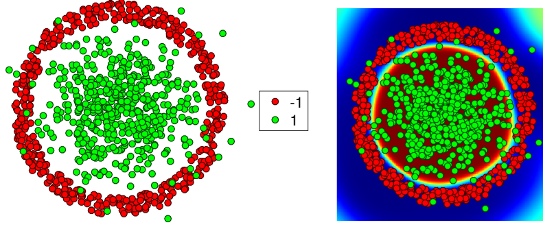
Figure 13.19. Nonlinear classification using a Gaussian kernel.
