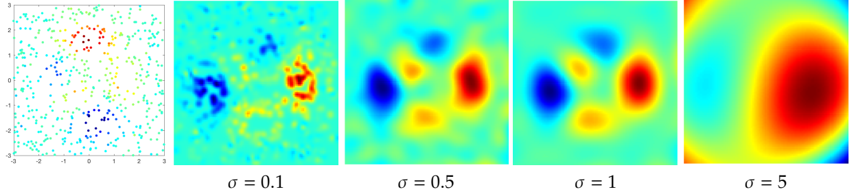
Figure 13.18. Regression using a Gaussian kernel.
