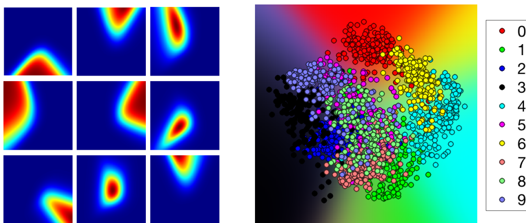
Figure 13.17. Digit classification results. Left: probability f(x, \hat{\beta})_\ell for each of the first nine classes, displayed in a 2-D PCA projection. Right: colors encode the class-probability vector f(x, \hat{\beta}) .
