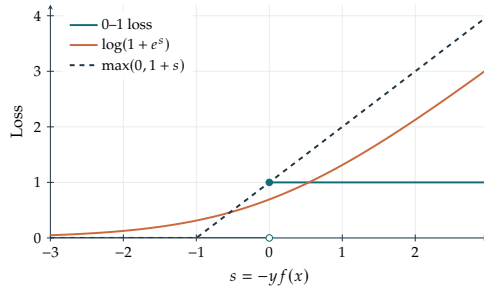
Figure 13.14. Classification losses as functions of the negative margin s = -y\langle x, \beta \rangle , with zero margin counted as an error. The unscaled logistic loss need not upper-bound the 0–1 loss; division by \log 2 gives the upper-bound normalization used above.
