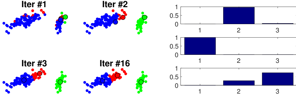
Figure 13.6. Left: iterations of the k -means algorithm. Right: class histograms after the k -means optimization.
