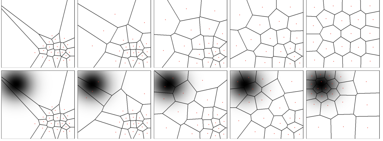
Figure 13.7. Continuous k -means (Lloyd) iterations for densities \mu . Top: uniform density. Bottom: nonuniform density, shown in grayscale as the density of \mu with respect to Lebesgue measure.
