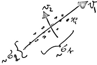
Figure 13.1. Empirical covariance of the data and its associated singular values.
