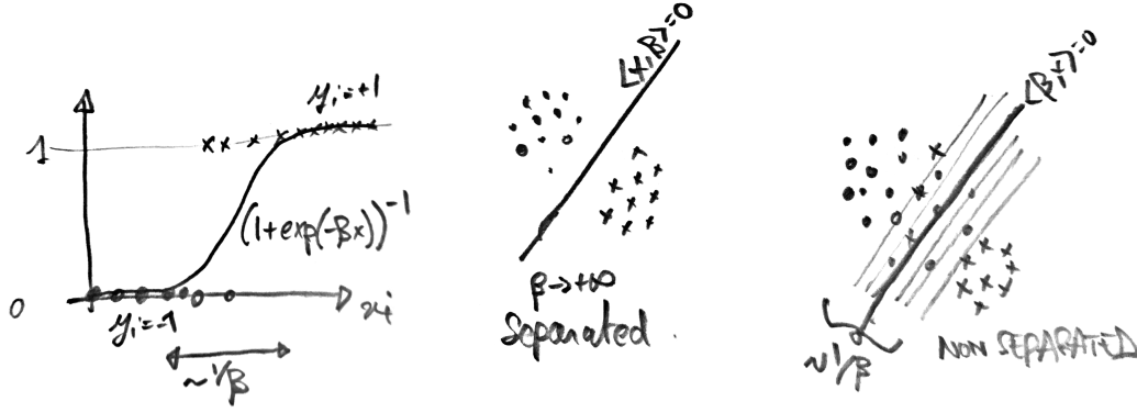
Figure 13.13. Logistic classification in one and two dimensions, showing how \|\beta\| controls the width of the probability transition.
