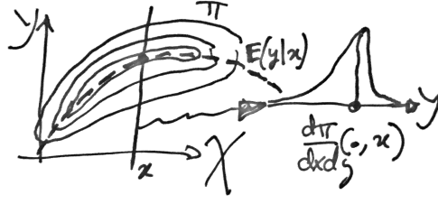
Figure 13.9. Conditional expectation.
