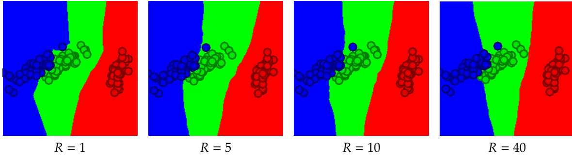
Figure 13.12. Classification boundaries produced by R -nearest neighbors.
