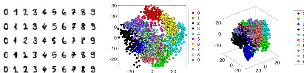
Figure 13.16. Digit images and their two- and three-dimensional PCA projections.
