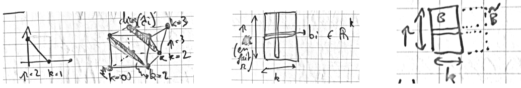
Figure 13.4. Left: the linear-program bound in (13.6). Middle: matrix B . Right: its orthogonal extension \tilde{B} .
