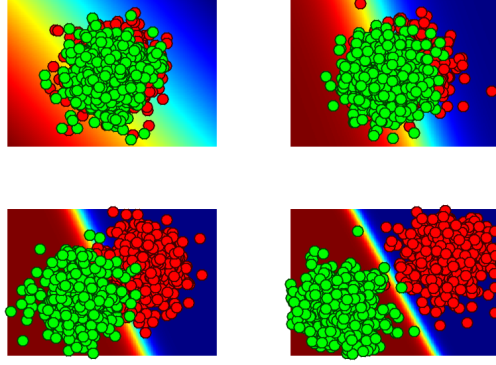
Figure 13.15. Effect of class separation on predicted classification probabilities.
