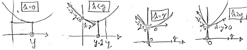
Figure 15.2. Effect of \lambda on the penalized scalar objective F(x) \stackrel{\text{def}}{=} \frac{1}{2}(x - y)^2 + \lambda|x| .
