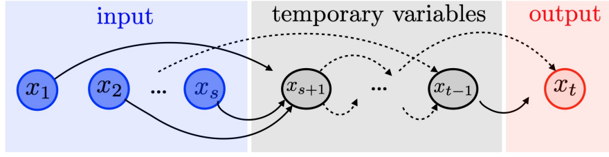
Figure 15.9. A computational graph.
