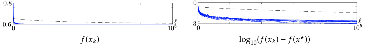
Figure 15.7. Objective-error evolution for SGD in logistic classification; the dashed curve shows batch gradient descent.
