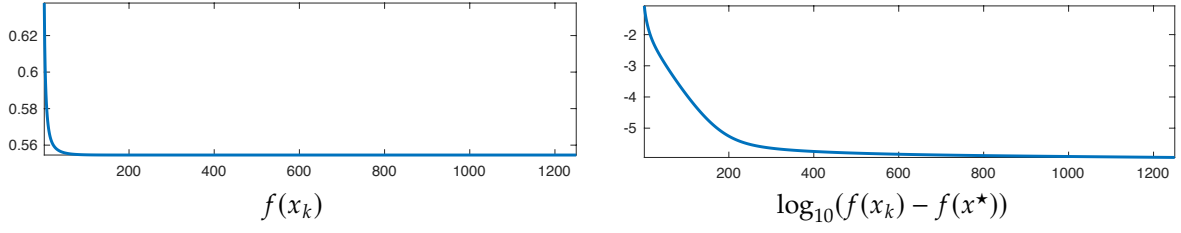
Figure 15.3. Objective-error evolution for batch gradient descent in logistic classification.
