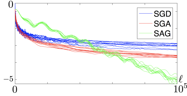
Figure 15.8. Evolution of \log_{10}(f(x_k) - f(x^*)) for SGD, SGA and SAG.
