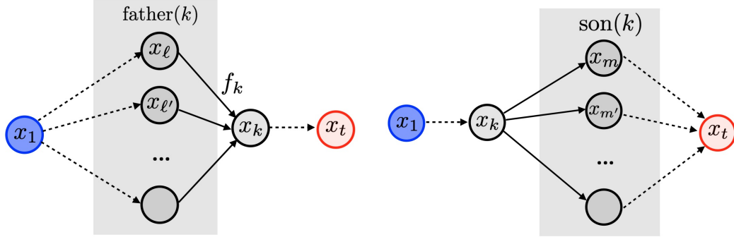
Figure 15.10. Derivative dependencies in forward mode (left) and reverse mode (right).
