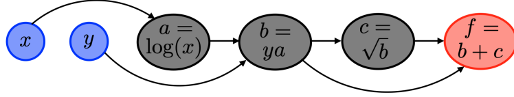
Figure 15.11. Example of a simple computational graph.
