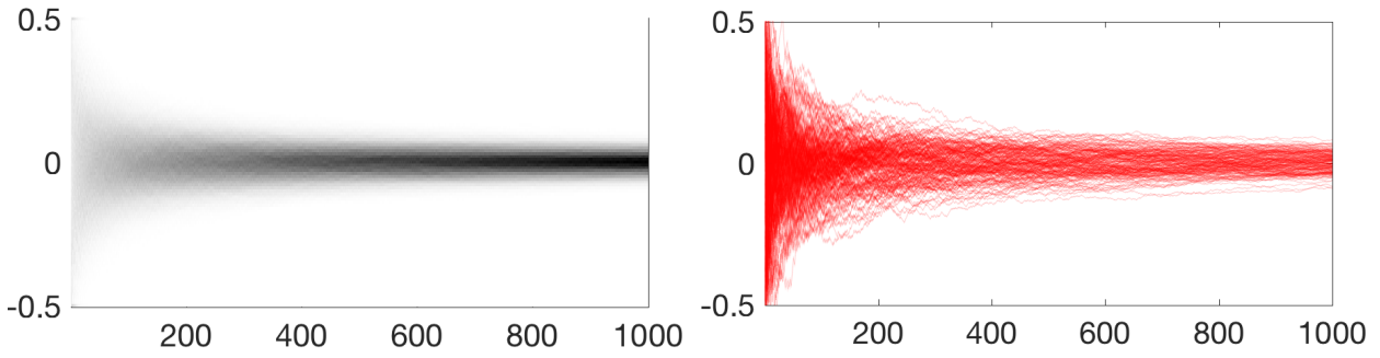
Figure 15.6. Repeated SGD runs for k \mapsto x_k \in \mathbb{R} . Left: the distribution of iterates at each iteration. Right: individual trajectories.
