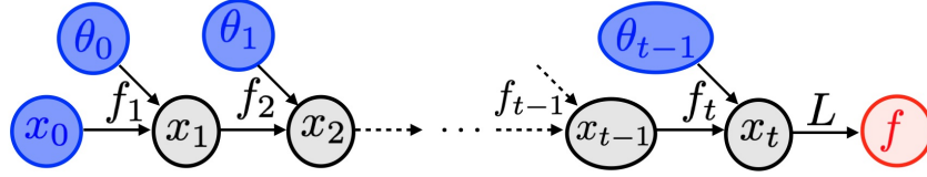
Figure 15.13. Computational graph for a feedforward architecture.
