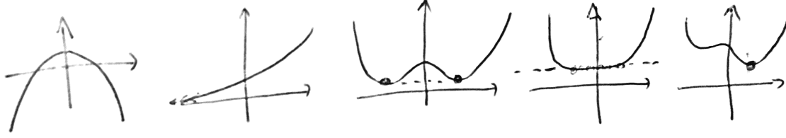
Figure 14.2. Left: no minimizer. Middle: multiple minimizers. Right: a unique minimizer.
