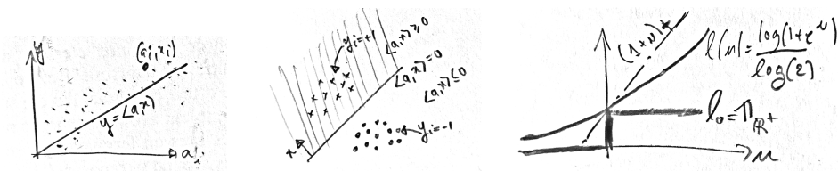
Figure 14.1. Left: linear regression. Middle: linear classifier. Right: classification loss.
