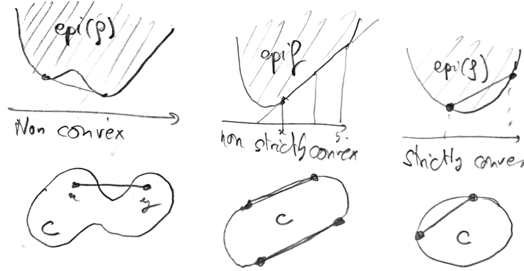
Figure 14.5. Comparison of convex functions f : \mathbb{R}^p \rightarrow \mathbb{R} (for p = 1 ) and convex sets C \subset \mathbb{R}^p (for p = 2 ).
