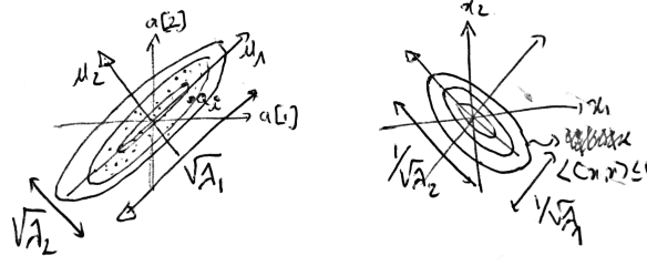
Figure 14.7. Left: point clouds (a_i)_i and their principal directions. Right: the quadratic part of f(x) .
