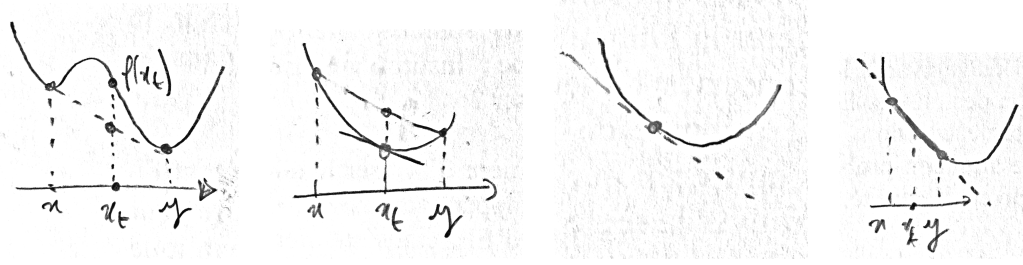
Figure 14.4. Convex and nonconvex functions; strictly convex and convex but not strictly convex functions.
