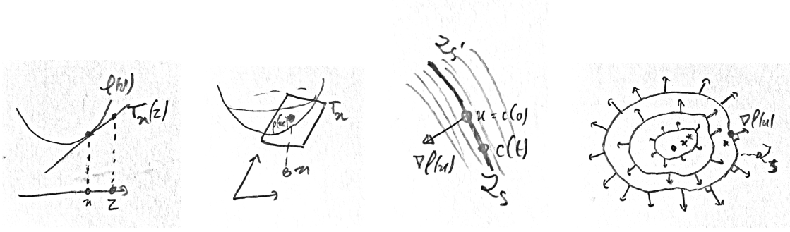
Figure 14.8. Left: first-order Taylor approximations in one and two dimensions. Right: the gradient is orthogonal to the level set; the diagram illustrates the proof.
