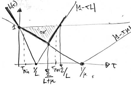
Figure 14.10. Contraction constant h(\tau) for a quadratic function.
