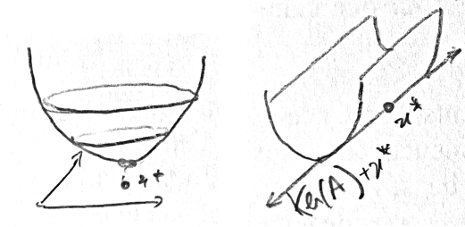
Figure 14.3. Coercivity condition for least squares.
