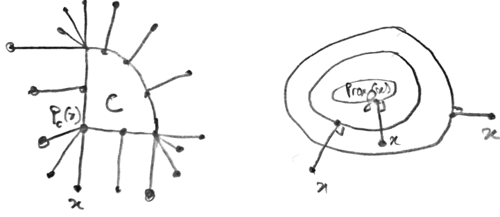
Figure 19.1. Proximal map and projection map.
