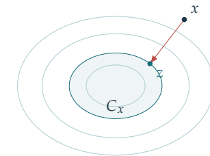
Projection onto an input-dependent sublevel set
