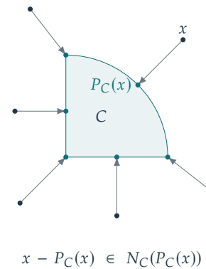
Projection onto a fixed set
