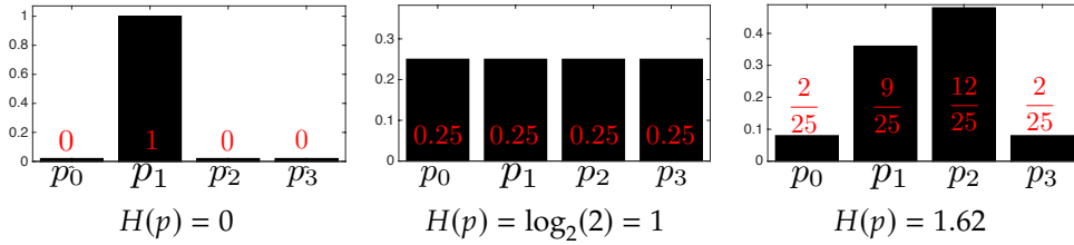
Figure 3.3. Three examples of probability distributions with corresponding entropies.
