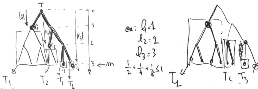
Figure 3.5. Left: full binary tree obtained by completing the tree associated with the code ( c_1 = 0, c_2 = 10, c_3 = 110, c_4 = 111 ). Right: subtrees with the prescribed codeword lengths packed from left to right.
