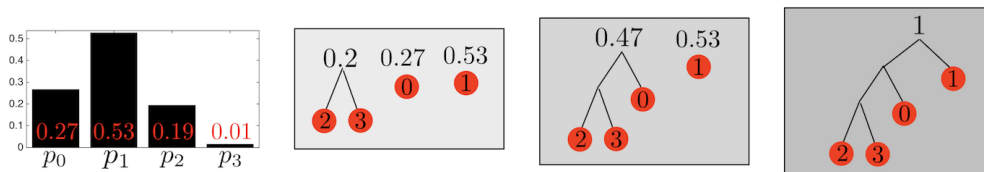
Figure 3.6. Successive merges in Huffman's coding algorithm.
