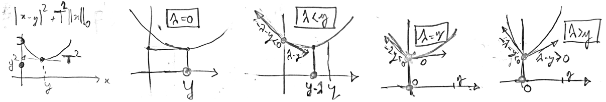
Figure 10.3. Left: the objective \|\cdot - y\|^2 + T^2 \|\cdot\|_0 . Remaining panels: the scalar objective F(x) \stackrel{\text{def.}}{=} \frac{1}{2} |x - y|^2 + \lambda |x| for increasing \lambda .
