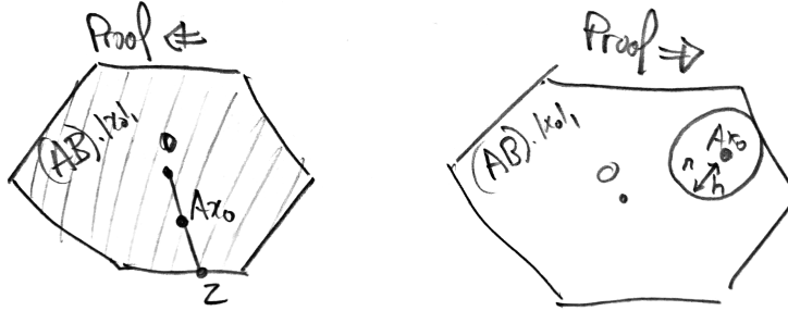
Figure 11.2. Geometry of the polytope characterization of exact recovery.
