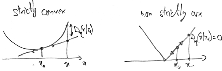
Figure 11.5. Visualization of Bregman divergences.
