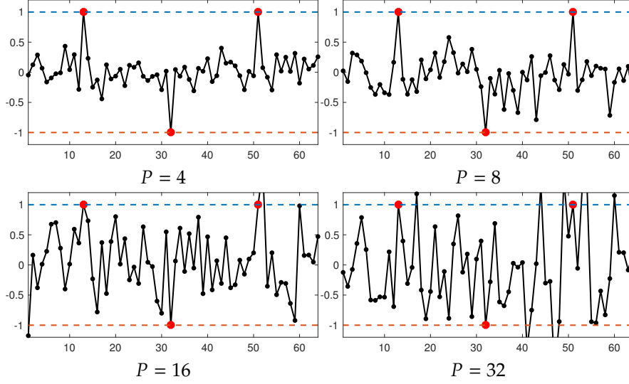
Figure 11.9. Fuchs precertificate \eta_F for a Gaussian matrix A \in \mathbb{R}^{P \times N} with N = 64 and increasing measurement count P .
