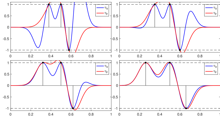
Figure 11.11. Continuous representations of the precertificates \eta_F and \eta_V for a convolution operator A .
