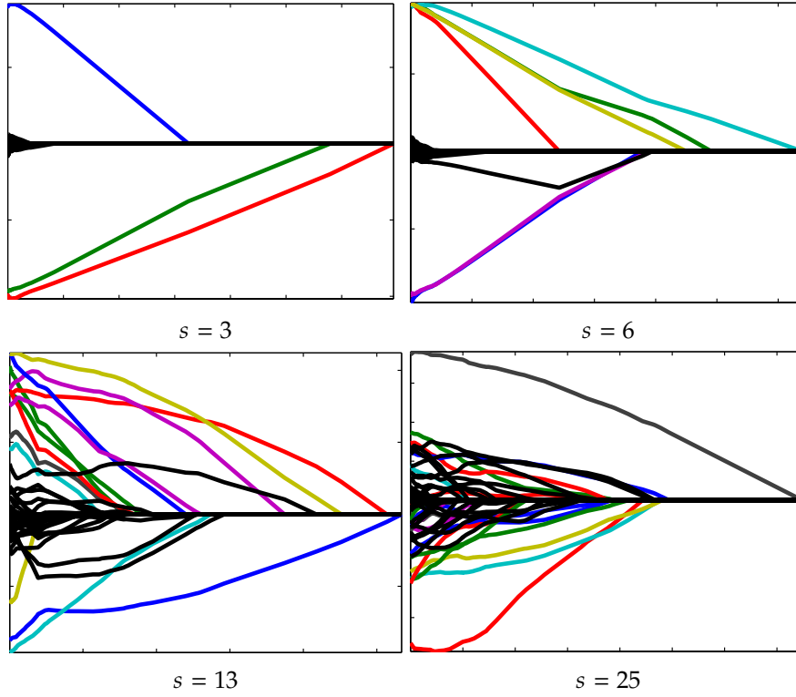
Figure 11.1. Solution paths \lambda \mapsto x_\lambda for (\mathcal{P}_\lambda(y)) .
