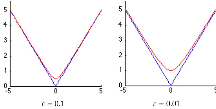
Figure 8.5. Regularized absolute value x \mapsto \sqrt{x^2 + \varepsilon^2} .
