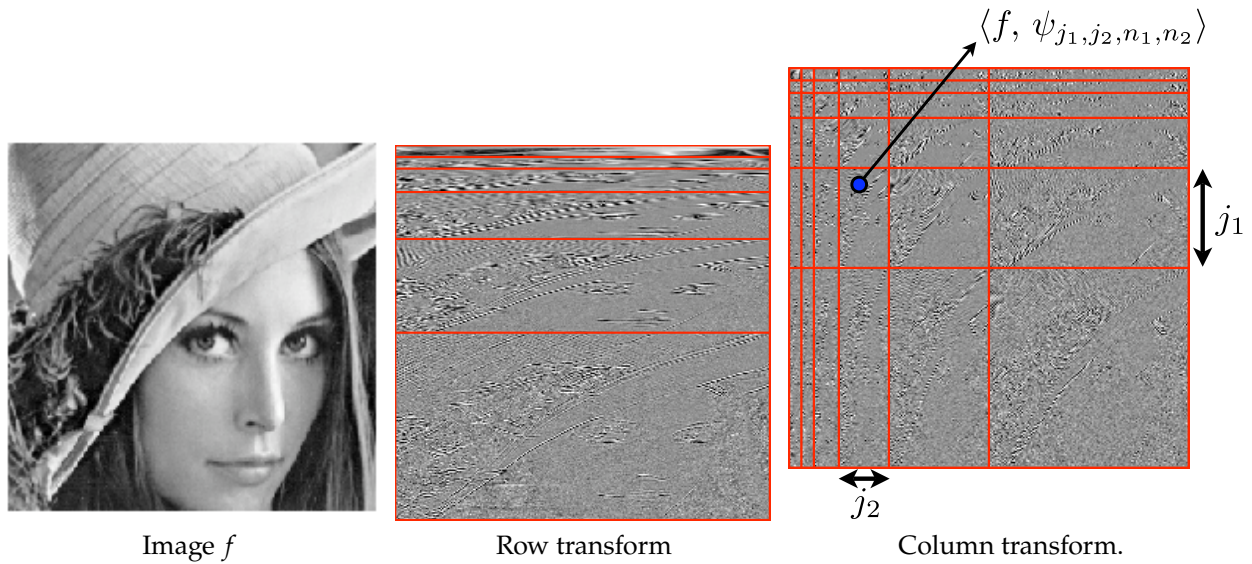
Figure 4.15. Steps of the anisotropic wavelet transform.
