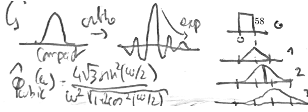
Figure 4.3. Orthogonalization of B-splines to define cardinal orthogonal spline functions.
