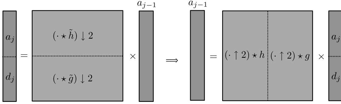
Figure 4.13. Inverse wavelet transform in matrix form.
