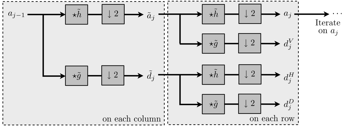
Figure 4.21. Forward 2-D filterbank step.
