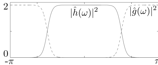
Figure 4.25. Complementarity of low-pass and high-pass filters h and g satisfying (\text{C}_3) .
