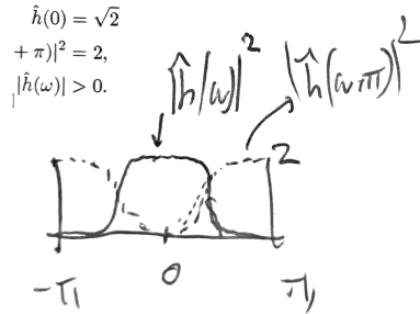
Figure 4.24. Constraints on low-pass and high-pass filters.
