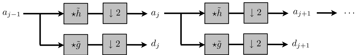
Figure 4.10. Forward filter bank decomposition.
