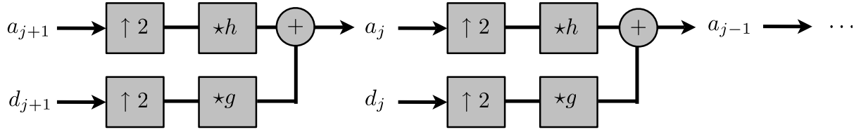
Figure 4.14. Inverse filter-bank reconstruction.
