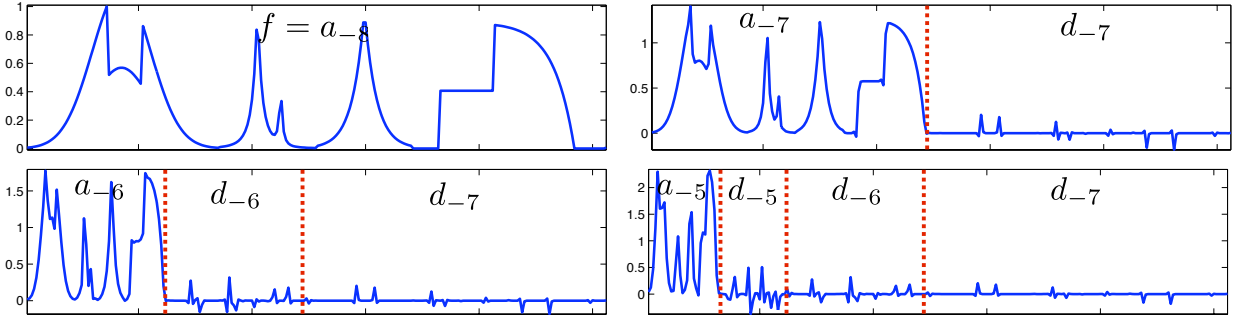
Figure 4.12. Wavelet decomposition algorithm.
