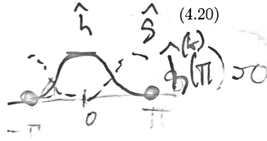
Figure 4.26. Vanishing moments correspond to vanishing derivatives of the Fourier transform.
