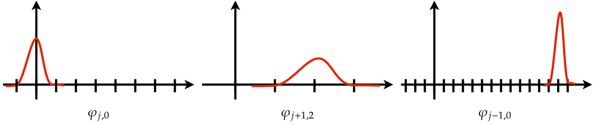
Figure 4.1. Translations and dilations of a scaling function generate the approximation spaces.
