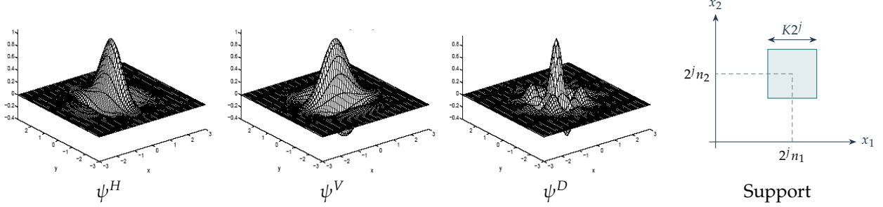
Figure 4.17. 2-D wavelets and a schematic support centered at (2^j n_1, 2^j n_2) , with width K2^j (right).
