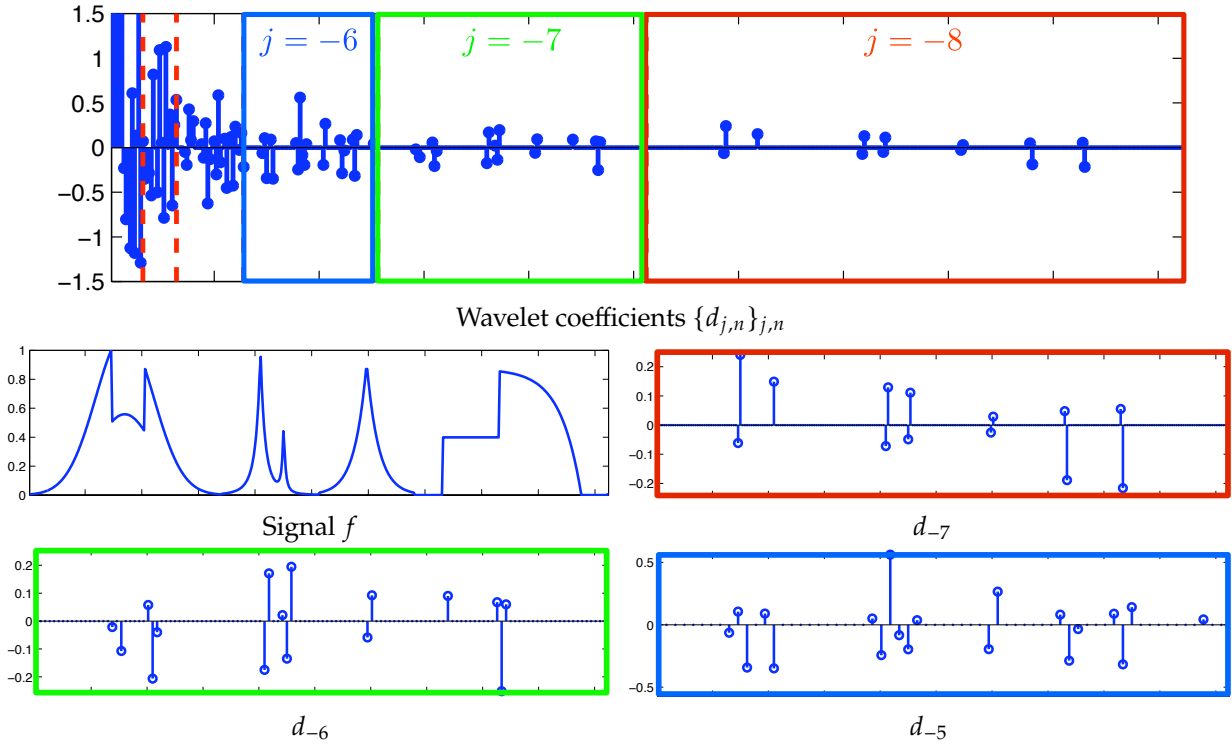
Figure 4.8. Wavelet coefficients. Top: the complete decomposition. Below: enlarged views of individual scales.
