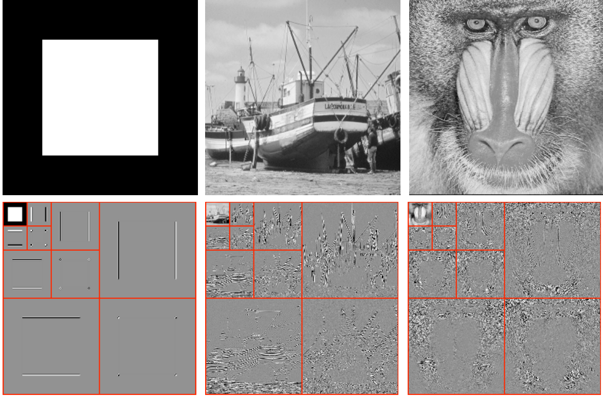
Figure 4.20. Images (top) and their wavelet coefficients (bottom).
