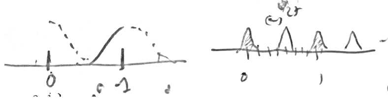
Figure 4.7. Periodized basis functions. Only the translations 0 \leq n < 2^{-j} are distinct, and j_0 = 0 is a common choice of coarsest scale.
