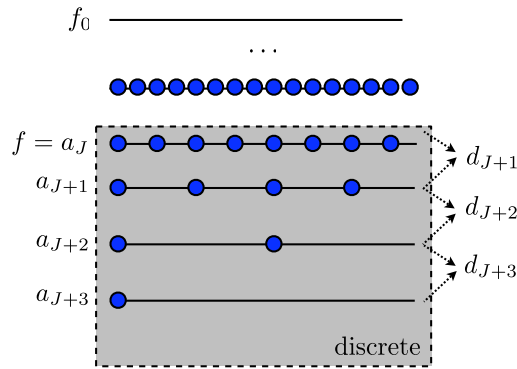
Figure 4.11. Pyramidal computation of wavelet coefficients.
