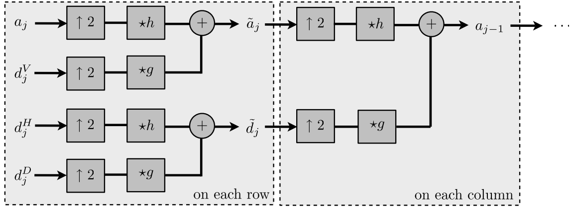
Figure 4.23. Backward 2-D filterbank step.
