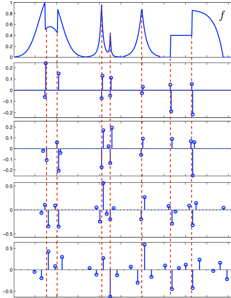
Figure 4.27. Location of large wavelet coefficients.
