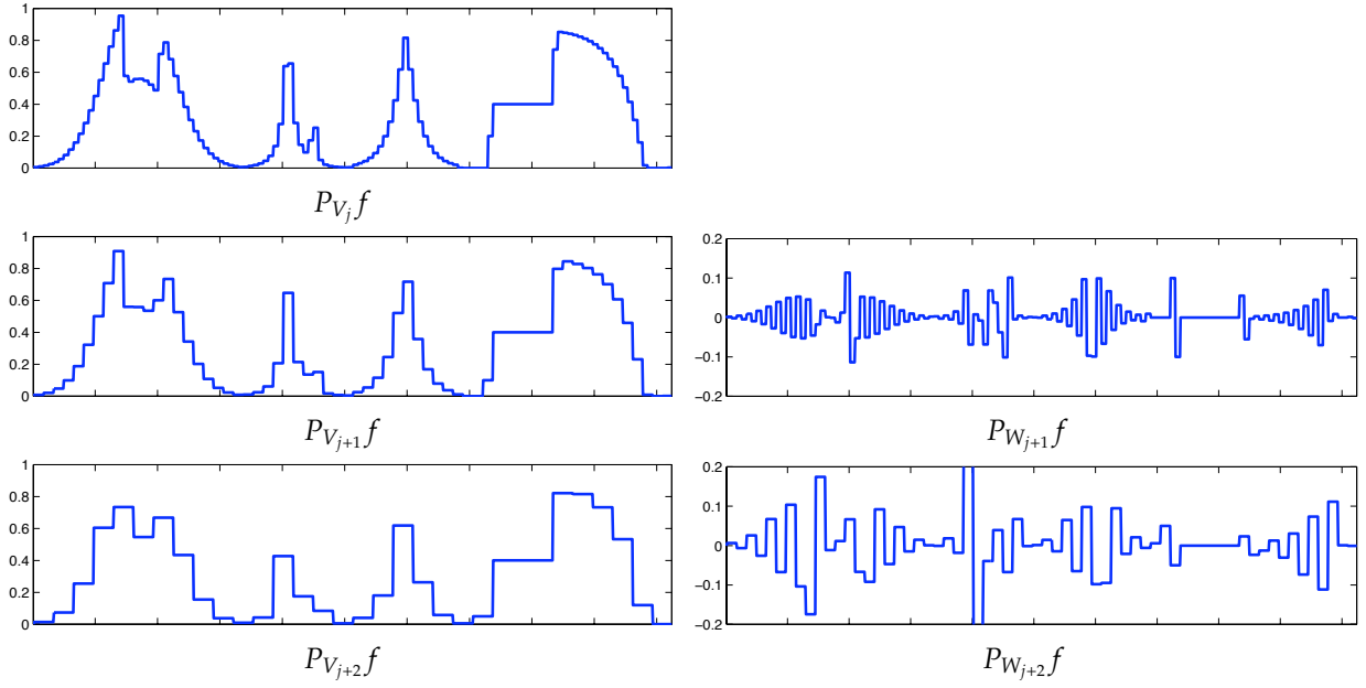
Figure 4.5. Successive Haar approximations (left) and the extracted details (right). Increasing the relative level from j to j + 1 and j + 2 coarsens the approximation.
