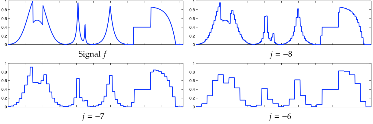
Figure 4.4. 1-D Haar multiresolution projection P_{V_j} f of a function f .
