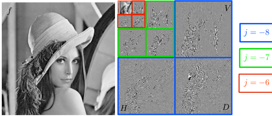
Figure 4.19. 2-D wavelet coefficients.
