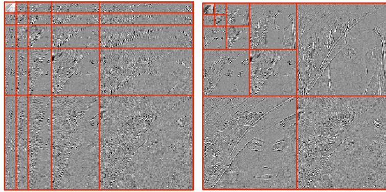
Figure 4.15. Steps of the anisotropic wavelet transform.
