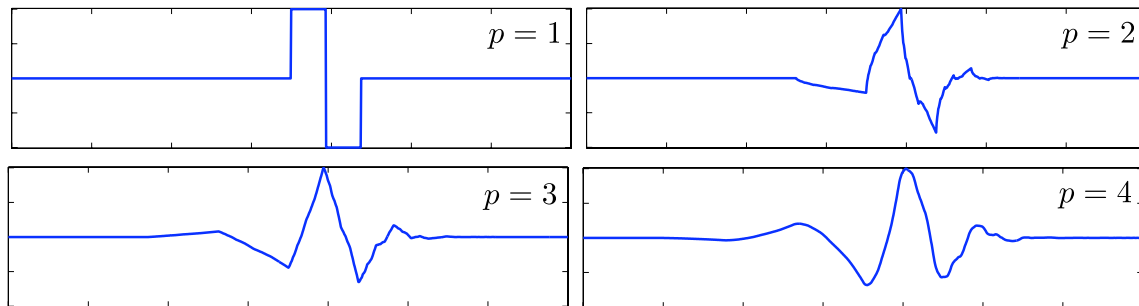
Figure 4.28. Daubechies mother wavelets \psi with increasing numbers p of vanishing moments.
