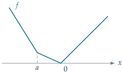
Piecewise affine convex function
