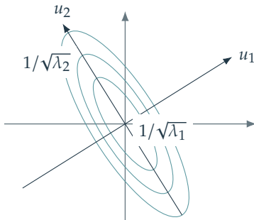
Quadratic level sets
