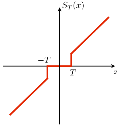
Figure 5.3. Hard thresholding.
