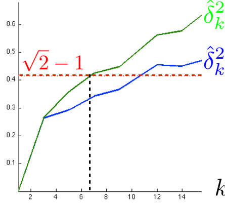
Figure 12.6. Evolution of lower bounds \hat{\delta}_k on the RIP constant.
