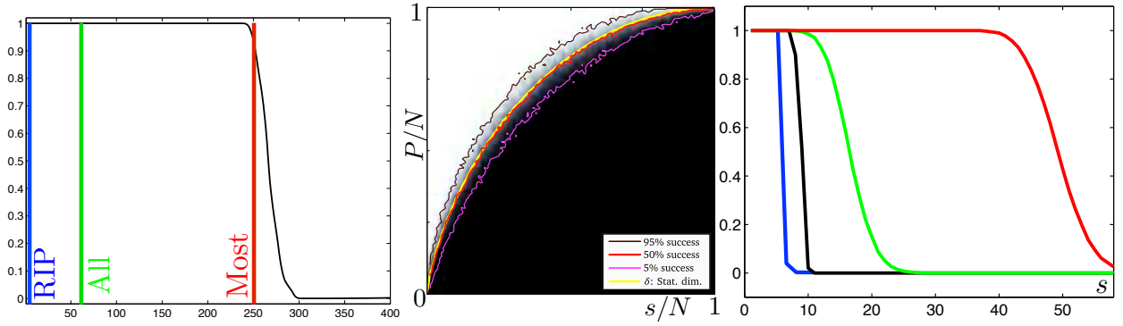
Figure 12.5. Phase transitions. Right: empirical probabilities that recovery criteria hold as sparsity varies. Blue: weak ERC; black: ERC; green: \|\eta_F\|_\infty \leq 1 ; red: exact recovery.
