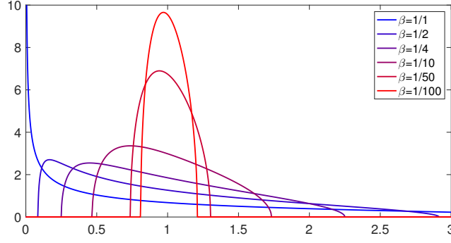
Figure 12.3. Marchenko–Pastur densities f_\beta for several aspect ratios \beta .
