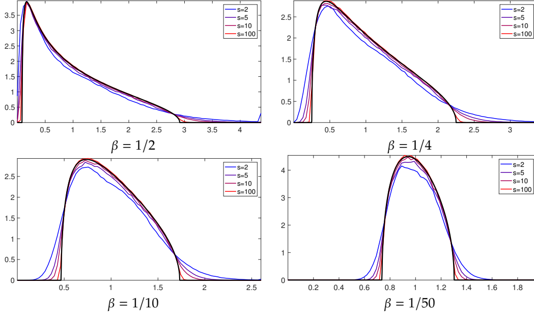
Figure 12.2. Empirical eigenvalue distributions approaching the Marchenko–Pastur law.
