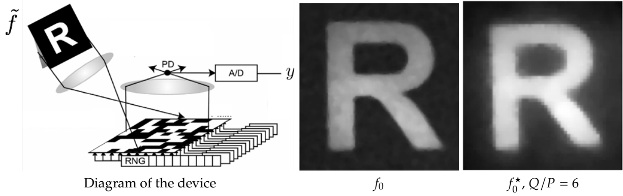
Figure 12.1. Left: diagram of the single-pixel acquisition method. Center: ideal image f_0 \in \mathbb{R}^Q in the micromirror focal plane. Right: reconstruction f_0^* = \Psi x^* from measurements y \in \mathbb{R}^P , with compression factor Q/P = 6 , using \ell^1 regularization.
