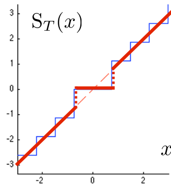
Figure 6.1. Hard thresholding and quantization as functions of the input coefficient.
