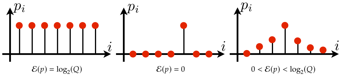
Figure 6.3. Three different probability distributions.
