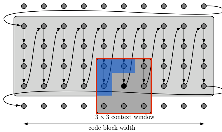
Figure 6.6. Coding order and context for JPEG-2000 coding.
