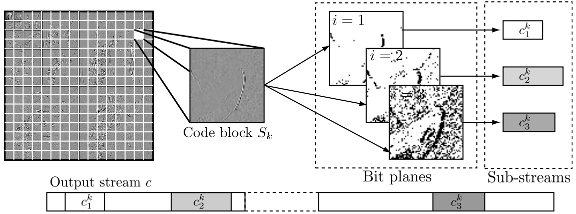
Figure 6.4. JPEG-2000 coding architecture.
