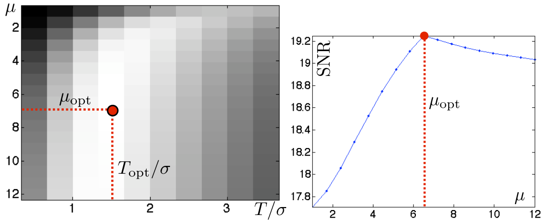
Figure 7.22. Left: SNR as a function of \mu and T/\sigma . Right: SNR versus \mu , with T/\sigma optimized separately for each \mu .
