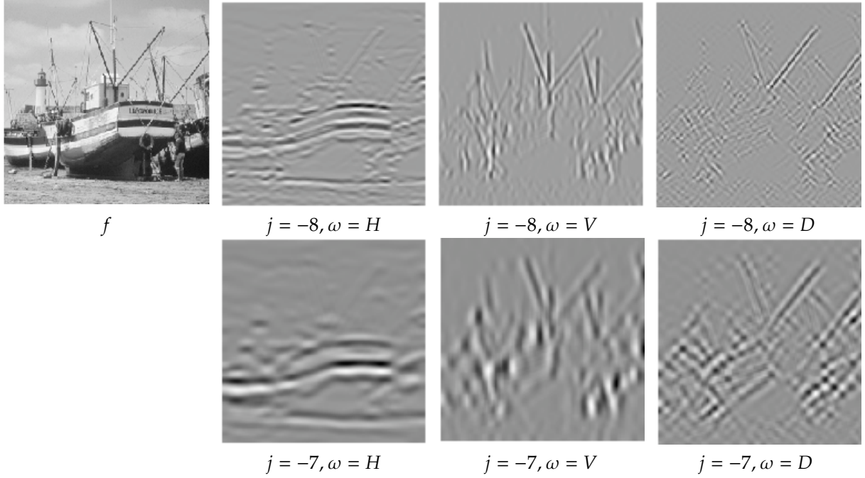
Figure 7.19. Translation invariant wavelet coefficients.
