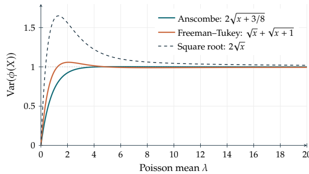
Figure 7.29. Exact Poisson variances of the Anscombe, Freeman–Tukey, and 2\sqrt{x} transforms as functions of the mean intensity.
