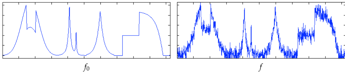
Figure 7.3. 1-D additive noise example.
