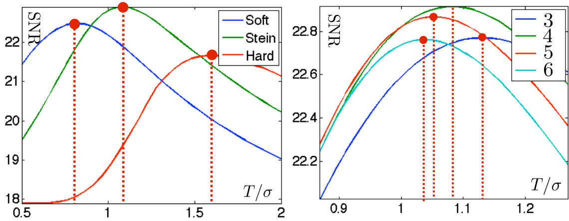
Figure 7.25. SNR as a function of T/\sigma (left) and comparison of different block sizes (right).
