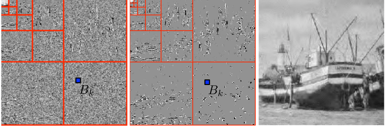
Figure 7.24. Left: wavelet coefficients, center: block thresholded coefficients, right: denoised image.
