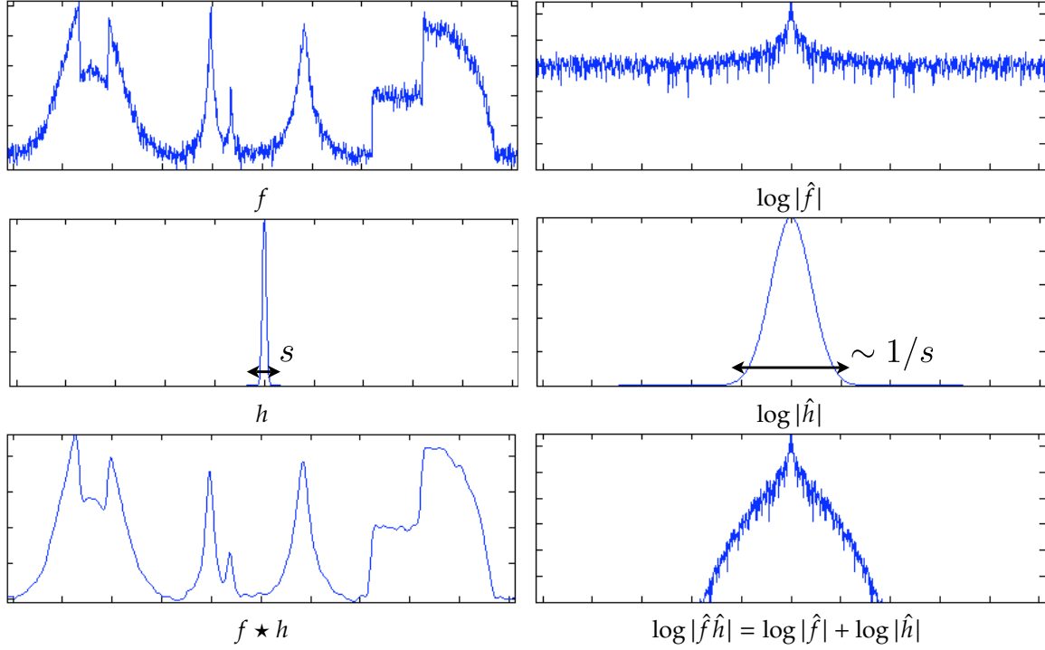
Figure 7.6. Filtering in the spatial domain (left) and the Fourier domain (right).
