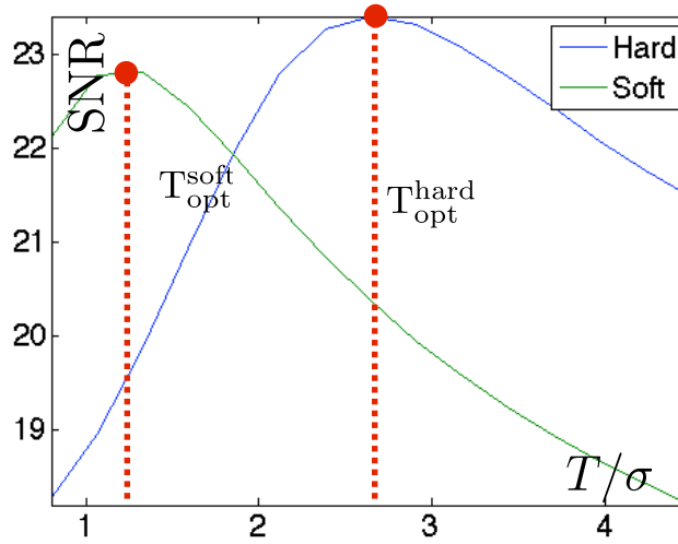
Figure 7.18. SNR as a function of T/\sigma for translation-invariant thresholding.
