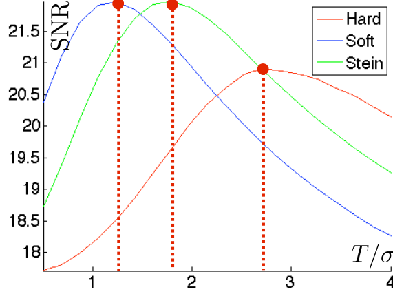
Figure 7.23. SNR as a function of T/\sigma for Stein thresholding.
