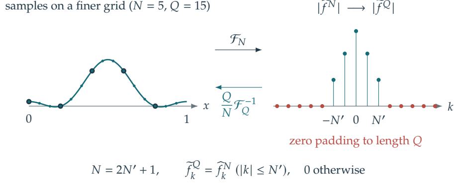
Figure 2.12. Interpolation by zero-padding in the frequency domain.
