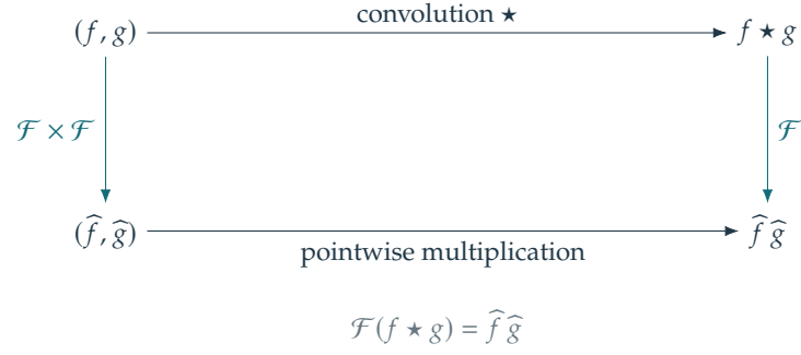
Figure 2.6. How the Fourier transform converts convolution into multiplication.
