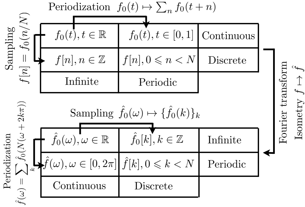
Figure 2.2. Four settings for Fourier analysis, linked by sampling and periodization.
