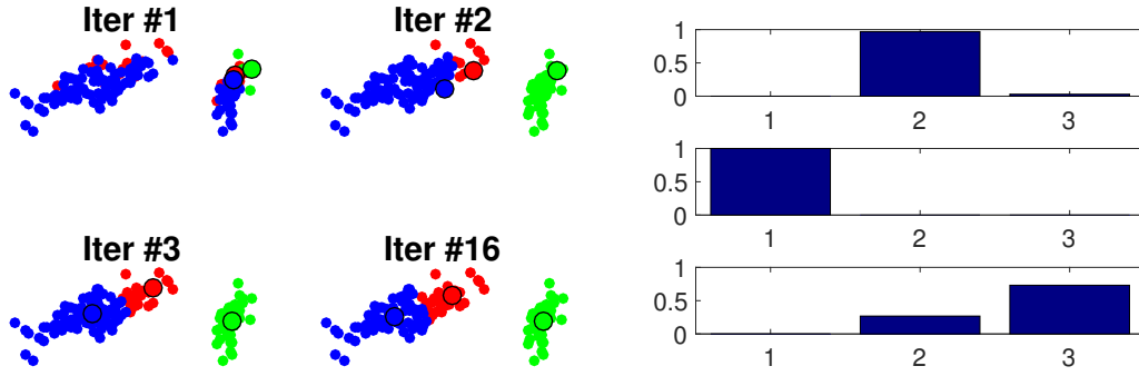
Figure 13.8. Left: iterations of the k -means algorithm. Right: class histograms after the k -means optimization.
