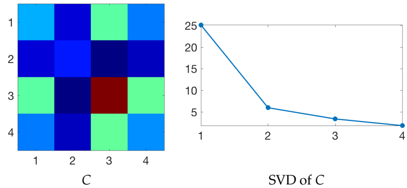
Figure 13.1. Empirical covariance of the data and its associated singular values.
