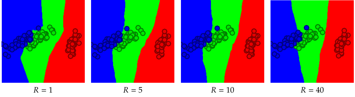
Figure 13.14. Classification boundaries produced by R -nearest neighbors.
