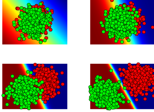
Figure 13.17. Effect of class separation on predicted classification probabilities.
