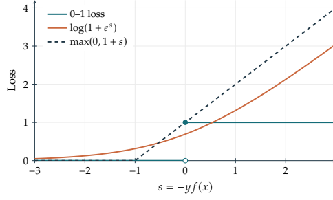
Figure 13.16. Classification losses as functions of the negative margin s = -y\langle x, \beta \rangle , with zero margin counted as an error. The unscaled logistic loss need not upper-bound the 0–1 loss; division by \log 2 gives the upper-bound normalization used above.
