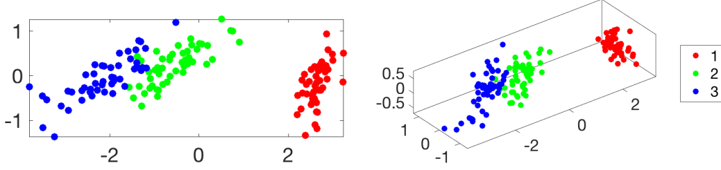
Figure 13.3. PCA projections of the data into two and three dimensions.
