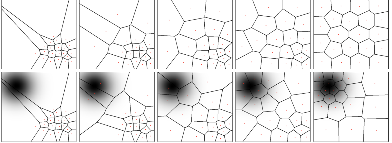
Figure 13.9. Continuous k -means (Lloyd) iterations for densities \mu . Top: uniform density. Bottom: nonuniform density, shown in grayscale as the density of \mu with respect to Lebesgue measure.
