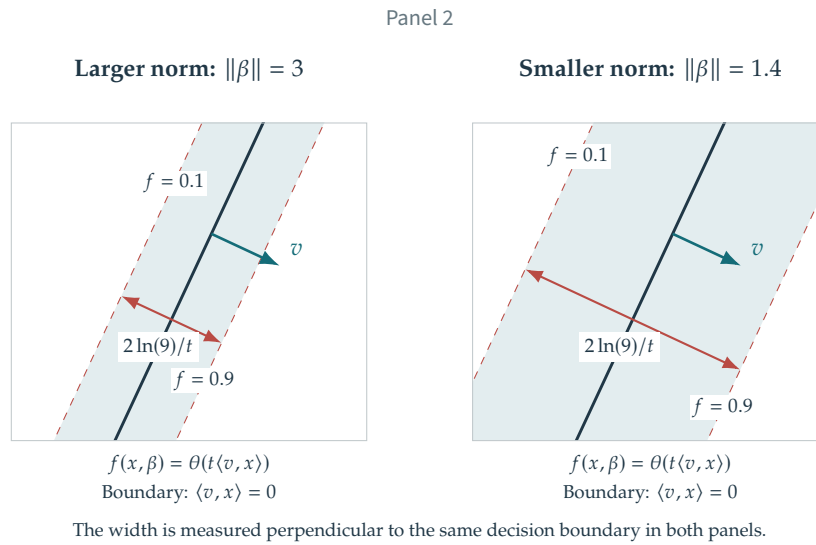
Figure 13.15. Logistic classification in one and two dimensions, showing how \|\beta\| controls the width of the probability transition.
