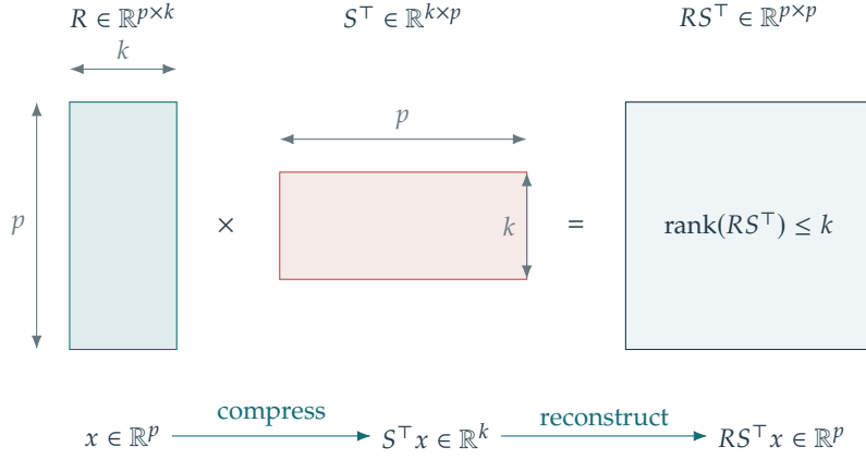
Figure 13.5. Linear compression followed by reconstruction.
