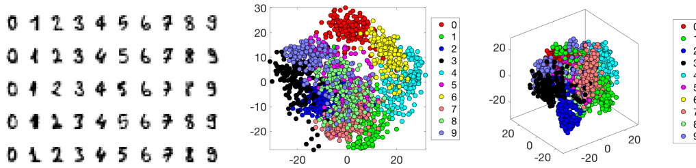
Figure 13.18. Digit images and their two- and three-dimensional PCA projections.
