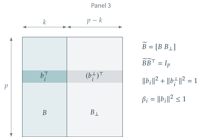
Figure 13.6. Panel 1: the linear-program bound in (13.6). Panel 2: matrix B . Panel 3: its orthogonal extension \tilde{B} .
