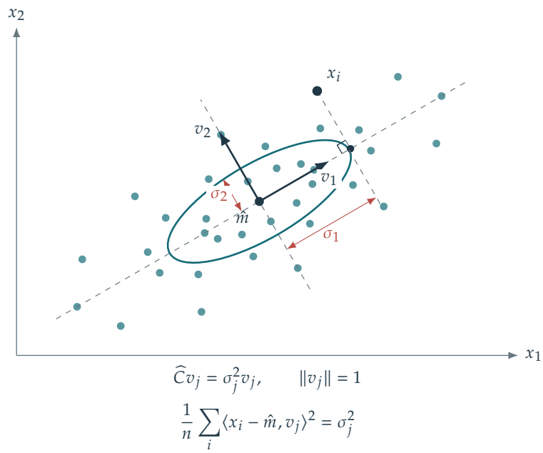
Figure 13.2. Principal directions of variation.
