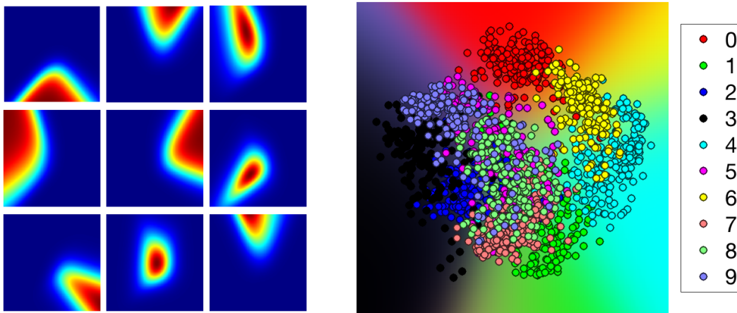
Figure 13.19. Digit classification results. Left: probability f(x, \hat{\beta})_\ell for each of the first nine classes, displayed in a 2-D PCA projection. Right: colors encode the class-probability vector f(x, \hat{\beta}) .
