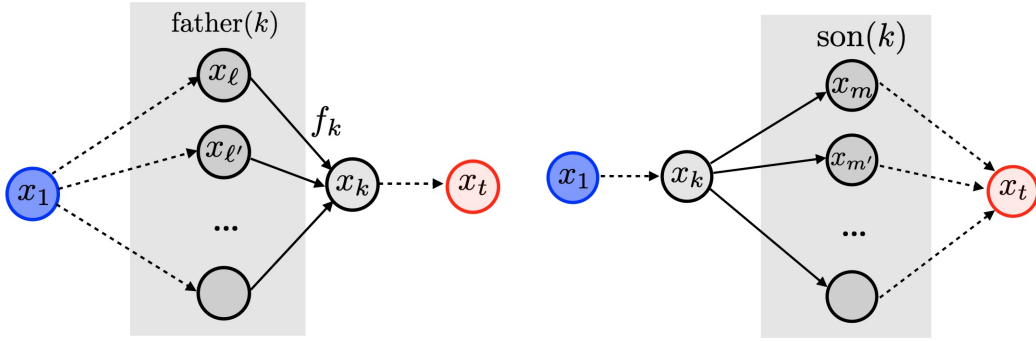
Figure 15.10. Derivative dependencies in forward mode (left) and reverse mode (right).
