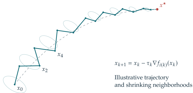
Figure 15.5. Schematic view of SGD iterates
