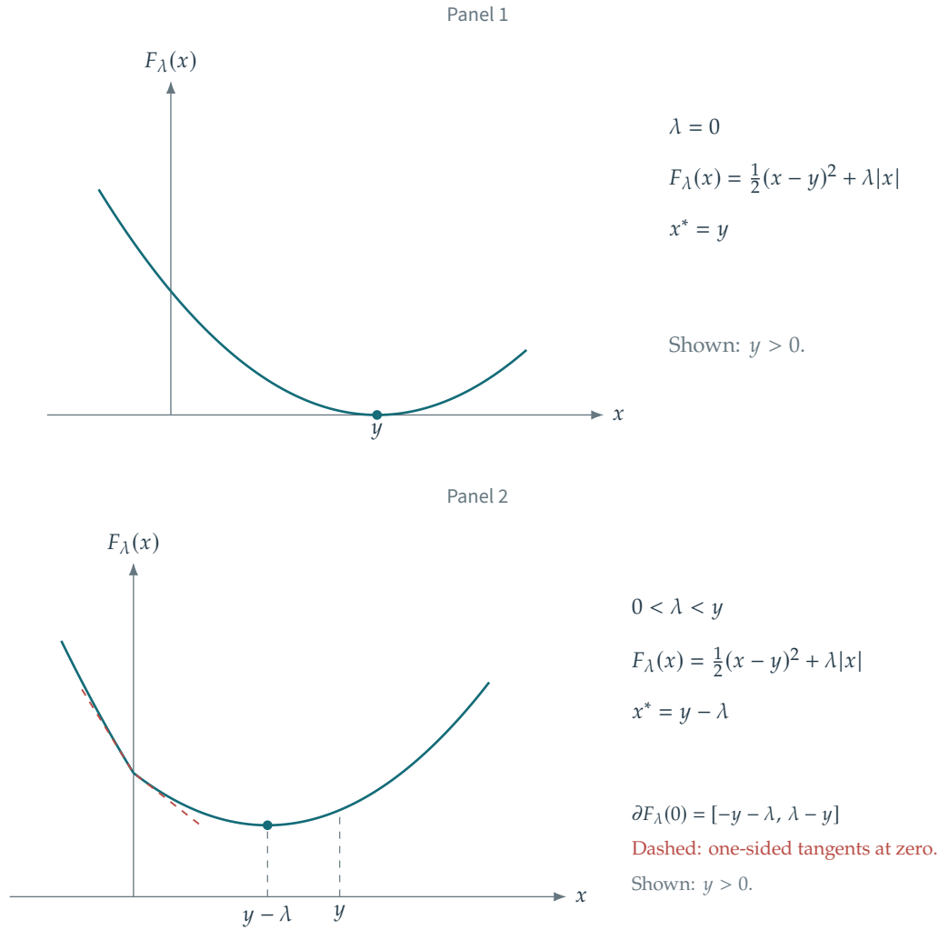
Figure 15.2. Effect of \lambda on the penalized scalar objective F(x) \stackrel{\text{def}}{=} \frac{1}{2}(x - y)^2 + \lambda|x| .
