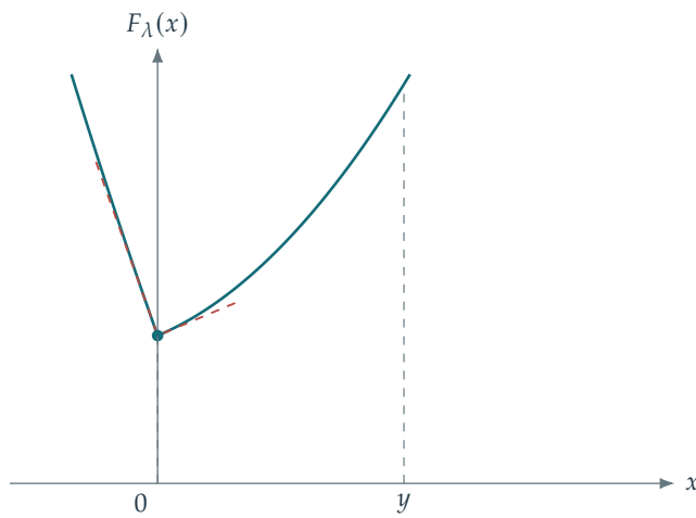
Figure 15.2 (continued). Effect of \lambda on the penalized scalar objective F(x) \stackrel{\text{def}}{=} \frac{1}{2}(x - y)^2 + \lambda|x| .
