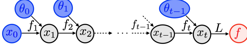
Figure 15.13. Computational graph for a feedforward architecture.
