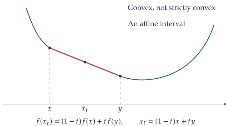
Figure 14.4 (continued). Convex and nonconvex functions; strictly convex and convex but not strictly convex functions.
