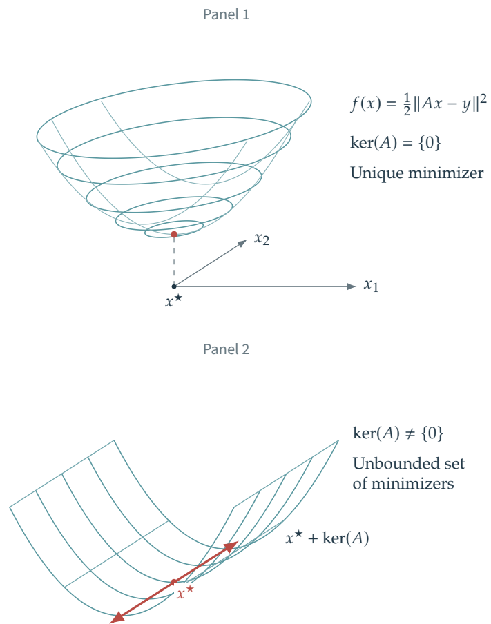
Figure 14.3. Coercivity condition for least squares.
