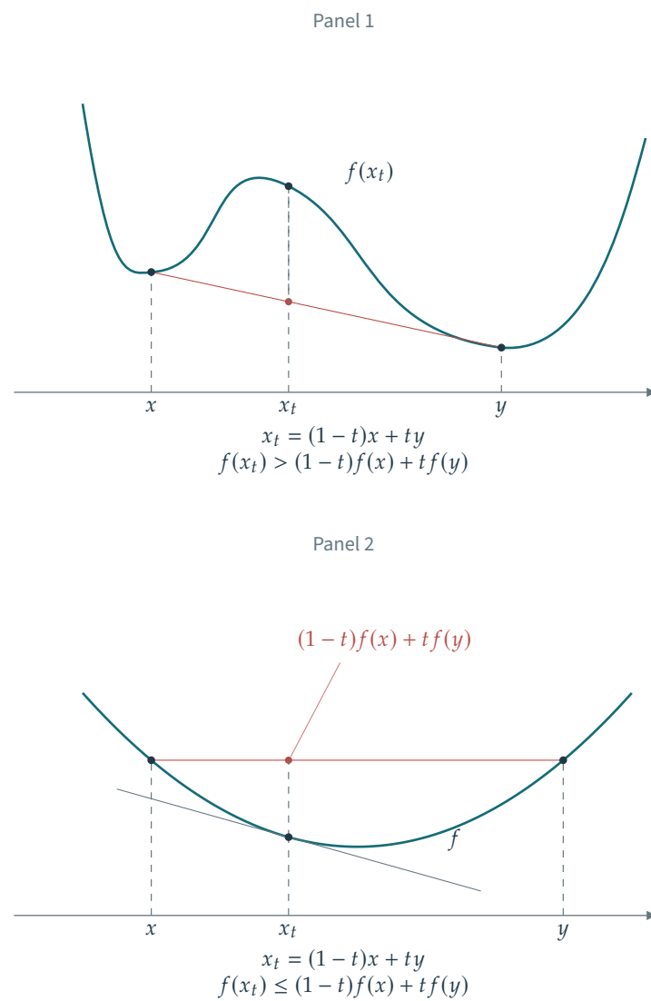
Figure 14.4. Convex and nonconvex functions; strictly convex and convex but not strictly convex functions.
