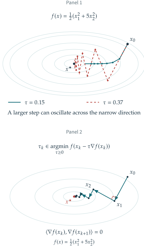
Figure 14.10. Effect of the step size \tau on gradient descent (panel 1) and exact line search (panel 2).
