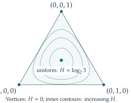
Three-symbol simplex
