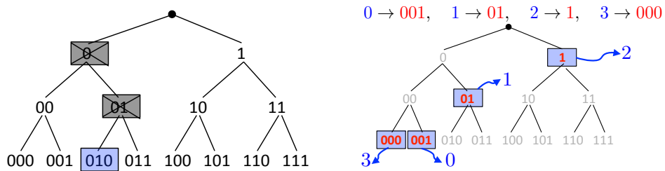
Figure 3.1. Left: the complete tree of binary words of length 3. Right: a prefix code.
